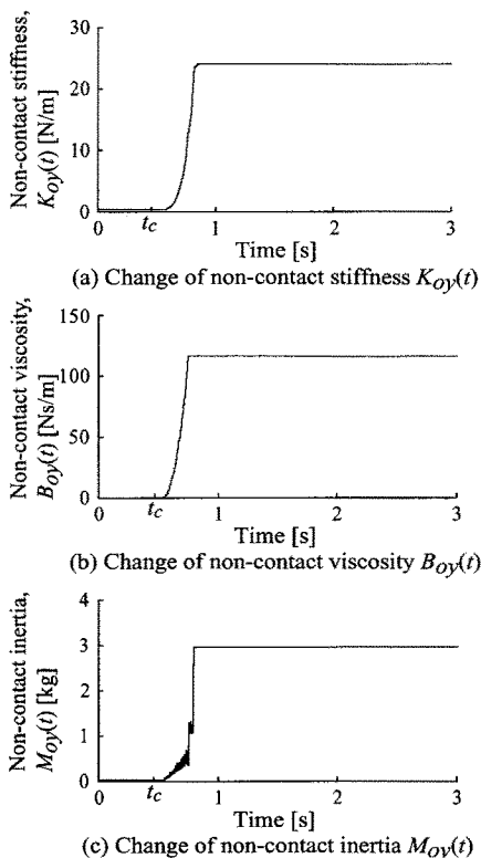
Fig. 9 Changes of the non-contact impedance parameters during the catching-a-ball task
