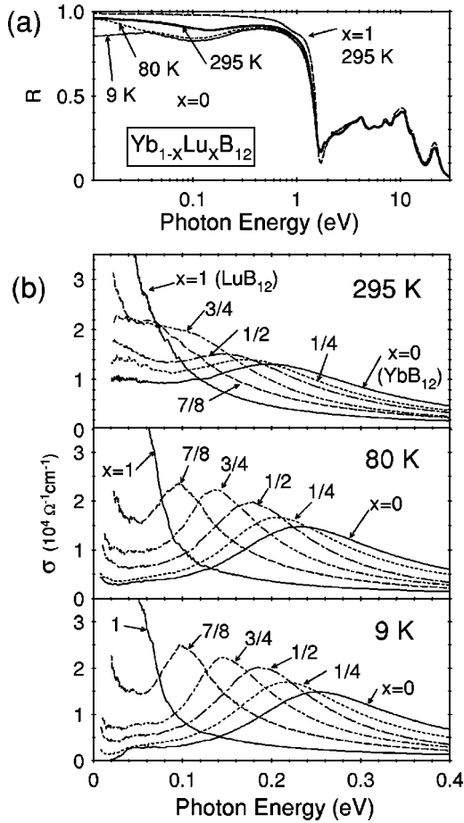
FIG. 1. Optical reflectivity ( R ) and conductivity ( \sigma ) spectra of \text{Yb}_{1-x}\text{Lu}_x\text{B}_{12} . (a) R of x=1 ( \text{LuB}_{12} ) at 295 K and those of x=0 ( \text{YbB}_{12} ) at 295, 80, and 9 K. (b) \sigma for various values of x at 295, 80, and 9 K.
