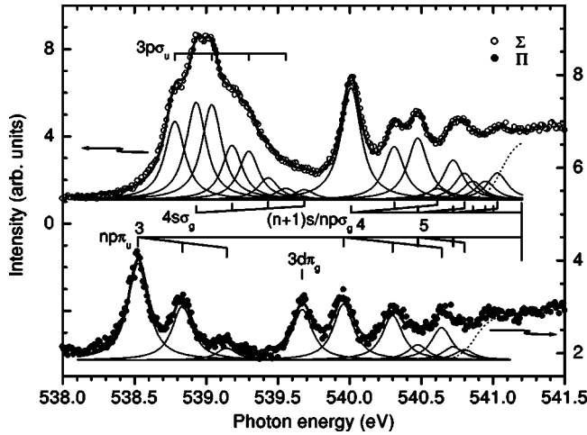
FIG. 2. \Sigma and \Pi spectra and the peak deconvolution analysis. The results of the fit are summarized in Tables I and II.
