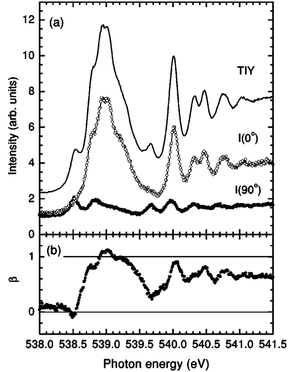
FIG. 1. The yield spectra and the anisotropy parameter \beta of photofragment ions of \text{CO}_2 in the region of the O 1s excitation to the Rydberg states. (a) Total-ion-yield spectrum and angle-resolved ion-yield spectra. (b) The \beta values of the energetic ions ( \geq 6 eV).
