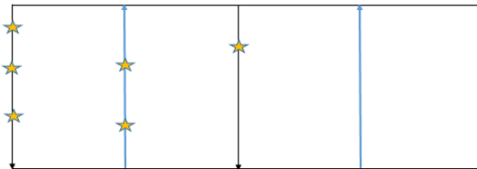
Figure 15: Skewed Distribution
