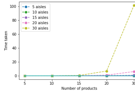
(f) Runtime (seconds)
