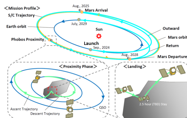
Figure 1. Overview of the MMX mission (credit JAXA)
