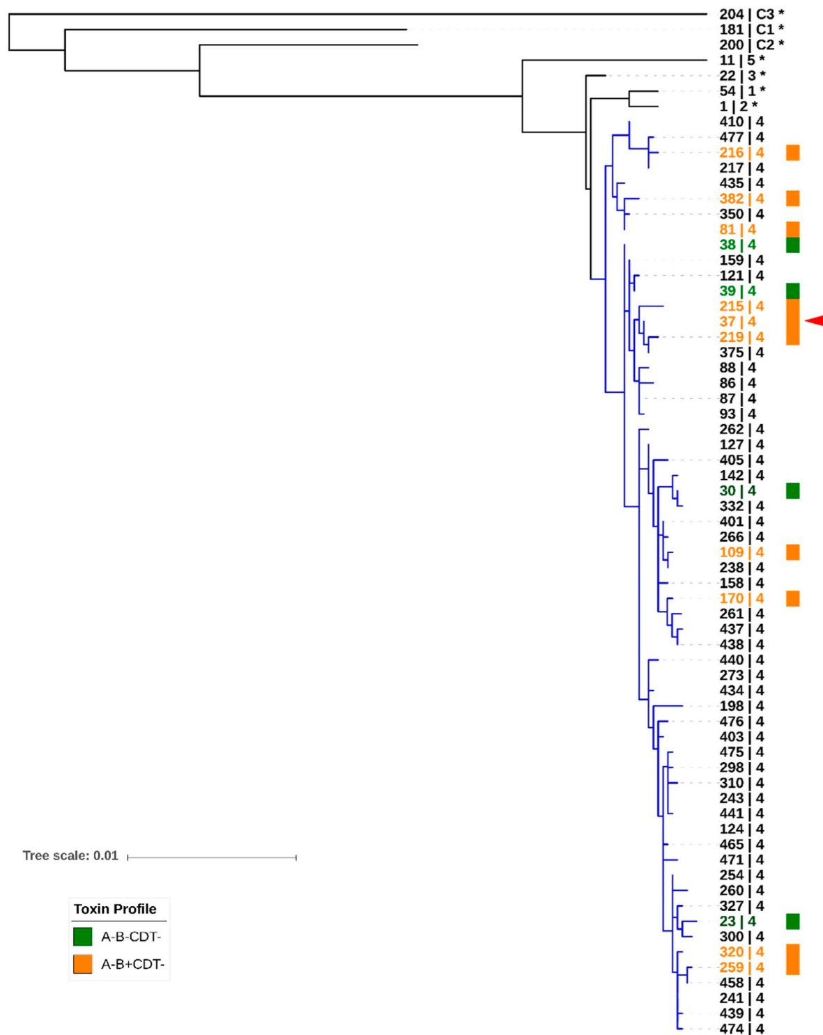
Figure 3. Sequence type diversity in evolutionary clade 4. Maximum-likelihood MLST phylogeny. Sequences were aligned using MUSCLE and tree was generated in MEGA7 with evolutionary distances calculated using the Tajima-Nei model. The scale shows the number of nucleotide substitution per site, based on concatenated MLST allele sequences (7 loci, 3501 bp). The tree is mid-point rooted and supported by 500 bootstrap replicates (only values >50 are shown). For global phylogenetic context, well-characterised representatives of MLST clade 1 (ST 54), 2 (ST 1), 3 (ST 22), 5 (ST 11), C1 (ST 181), C2 (ST 200), and C3 (ST 204) are also shown (*). Branches for clade 4 are shown in blue. Known toxin profiles of clade 4 strains are indicated by orange (A-B+CDT-) and green (A-B-CDT-) colour. RT 017 (ST 37) is indicated with a red arrowhead.
