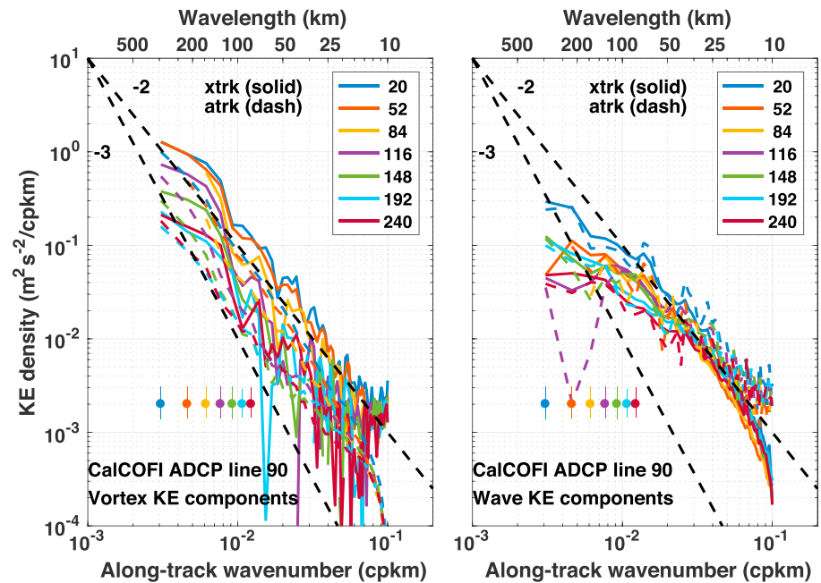
Figure 8. Spectra of vortex (left) and wave (right) kinetic energy (KE) components for acoustic Doppler current profiler (ADCP) transects along line 90. Solid lines denote across-track components, and dashed lines denote along-track components. Depths are differentiated by color. The 95% confidence limits are shown, color coded by depth. Black dashed lines show slopes of -2 and -3 for reference. CalCOFI = California Cooperative Oceanic Fisheries Investigations.
