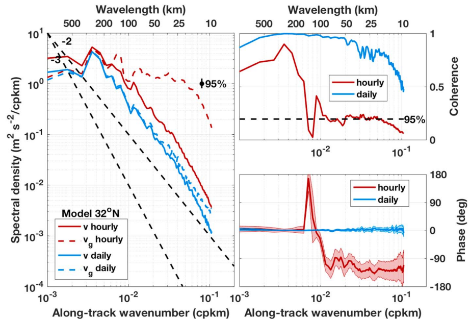
Figure 15. (left) Spectral density of meridional velocity v (colored solid lines) and geostrophic velocity v_g (colored dashed lines) estimated from the latitude-longitude cap 4320 model along latitude 32^\circ\text{N} in the subdomain shown in Figure 3. Black dashed lines show slopes of -2 and -3 for reference. (upper right) Coherence between v and v_g ; 95% significance level is shown by the black dashed line. (lower right) Phase between v and v_g ; 95% confidence is denoted by shading. In all panels, values corresponding to hourly and daily averaged velocities are denoted by red and blue, respectively.
