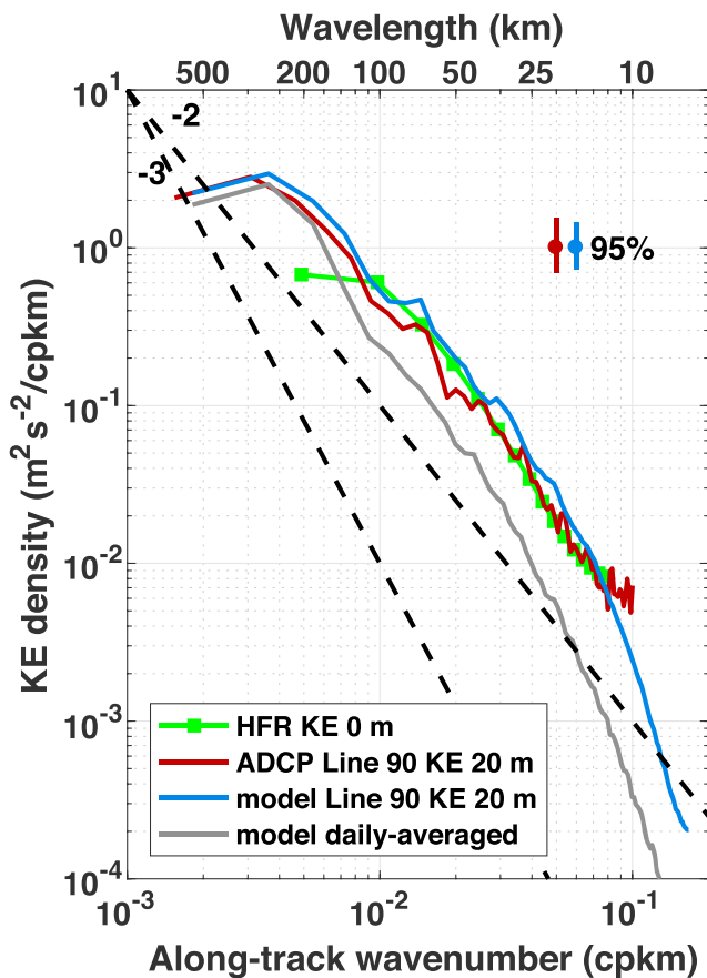
Figure 4. Kinetic energy (KE) spectra at 20-m depth for acoustic Doppler current profiler (ADCP; red) and latitude-longitude cap 4320 model-hourly (blue) and model-daily (gray) transects along line 90. Also shown, the KE surface spectrum (green) from high-frequency radar (HFR) estimated by Kim et al. (2011) for the region denoted by the green box shown in Figure 1. The 95% confidence limits are shown for the ADCP (red) and model-hourly (blue) estimates. Black dashed lines show slopes of -2 and -3 for reference.
