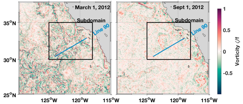
Figure 3. Snapshots of surface relative vorticity from the latitude-longitude cap 4320 model taken at midnight UTC on 1 March (left) and 1 September 2012 (right). The blue line corresponds to CalCOFI Line 90. Model kinetic energy spectra are estimated along this line for comparison with observations. Model velocity gradient statistics are estimated for the subdomain denoted by the black box.
