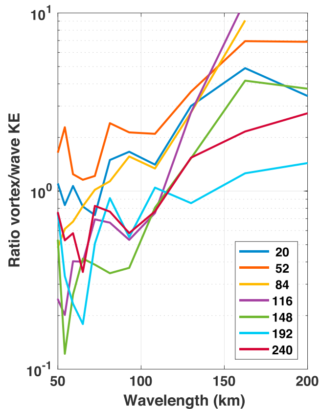
Figure 9. Ratio of vortex:wave kinetic energy (KE) versus wavelength at multiple depths for the acoustic Doppler current profiler vortex-wave decompositions shown in Figure 8. Ratios larger than 1 are interpreted as dominated by balanced (geostrophic) motions; ratios less than 1 are interpreted as dominated by ageostrophic motions.
