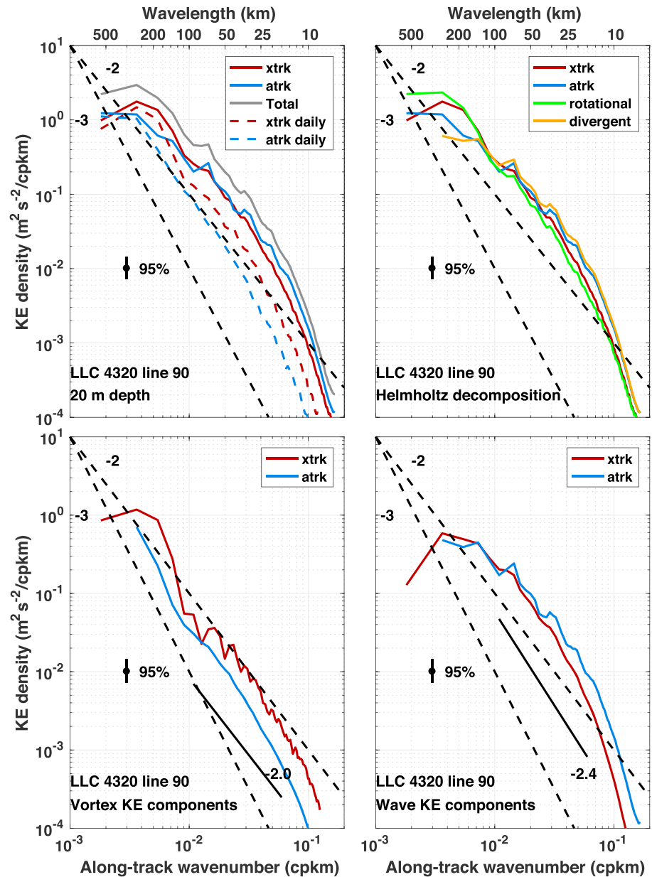
Figure 6. Helmholtz and wave-vortex decompositions of the LLC 4320 model-hourly KE spectra at 20-m depth along line 90. (upper left) Across-track (red) and along-track (blue) KE components at 20-m depth for model-hourly (solid) and model-daily (dashed) transects. Total (gray) model-hourly KE as shown by the blue line in Figure 4. (upper right) Across-track (red) and along-track (blue) KE components and the Helmholtz decomposition into rotational (green) and divergent (orange) components. (lower left) Vortex across-track (red) and along-track (blue) components. (lower right) Wave across-track (red) and along-track (blue) components. In all panels, black dashed lines show slopes of -2 and -3 for reference; 95% confidence limits are also shown. In the lower panels, the slope of the solid black line is a least squares fit to the KE estimates over the wavenumber range 0.01 to 0.06 cpkm, offset for clarity. KE = kinetic energy; LLC = latitude-longitude cap.
