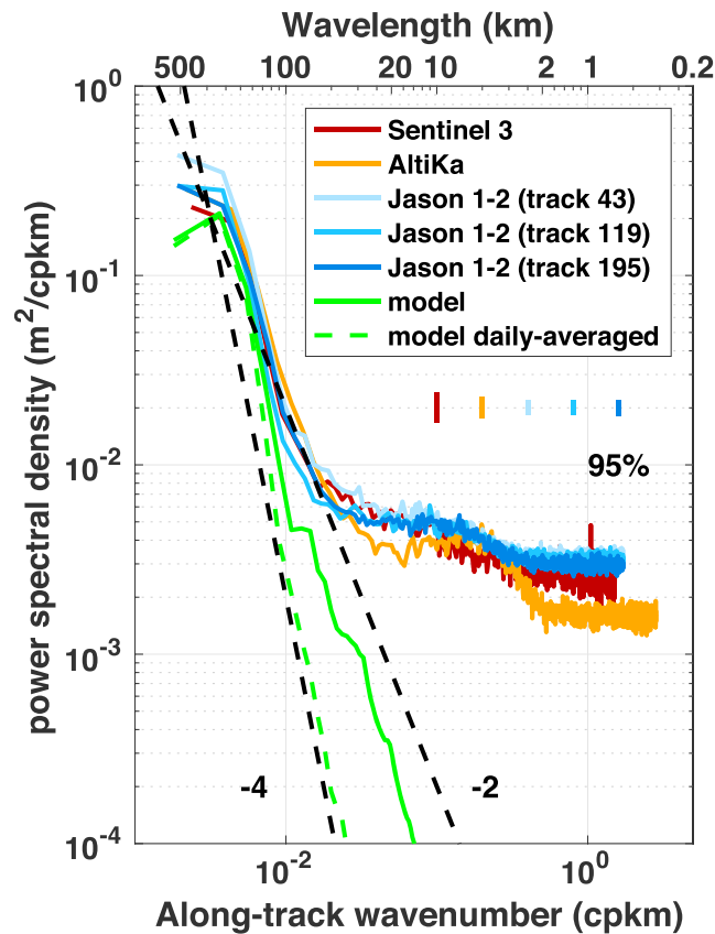
Figure 14. Sea surface height spectra for the California Current altimeter tracks shown in Figure 2 and for the latitude-longitude cap 4320 model output. For reference, black lines indicate k^{-2} and k^{-4} spectral slopes.
