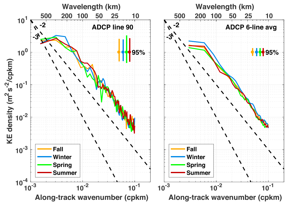
Figure 12. Seasonal averages of total kinetic energy (KE) at 20-m depth for (left) acoustic Doppler current profiler (ADCP) transects along line 90 and (right) ADCP transects averaged over all six CalCOFI lines. In both panels transects were averaged according to seasons: fall (September/October/November), winter (December/January/February), spring (March/April/May), and summer (June/July/August). The 95% confidence limits are shown, color coded by season. Black lines show slopes of -2 and -3 for reference.
