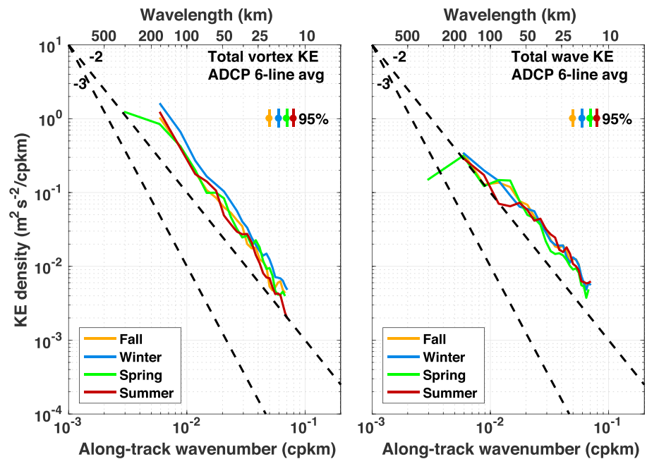
Figure 13. Seasonal averages of total kinetic energy (KE) decomposed into vortex (left) and wave (right) contributions for acoustic Doppler current profiler (ADCP) transects at 20-m depth averaged over all six CalCOFI lines. Transects were averaged according to seasons: fall (September/October/November), winter (December/January/February), spring (March/April/May), and summer (June/July/August). The 95% confidence limits are shown, color coded by season. Black lines show slopes of -2 and -3 for reference.
