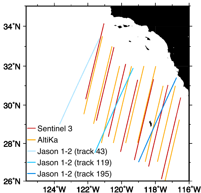
Figure 2. Altimeter ground track segments used for this study, including tracks from Jason-1 and Jason-2 (blue), Sentinel-3 (red), and AltiKa (orange). Sentinel-3 and AltiKa tracks are descending (collected when the satellite is moving southward), and Jason tracks are ascending (satellite moving northward).
