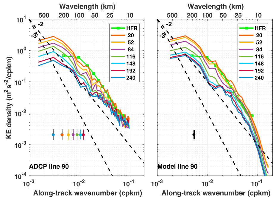
Figure 7. Total kinetic energy (KE) estimates for acoustic Doppler profiler (ADCP; left) and latitude-longitude cap 4320 model-hourly (right) transects along line 90 are shown for a subset of depth layers. The total KE surface spectrum from high-frequency radar (HFR) was estimated by Kim et al. (2011) for the region denoted by the green box shown in Figure 1 and is plotted in both panels. The 95% confidence limits are shown for the acoustic Doppler current profiler (left, color coded for depth) and model (right, hourly averaged data). Black dashed lines show slopes of -2 and -3 for reference.
