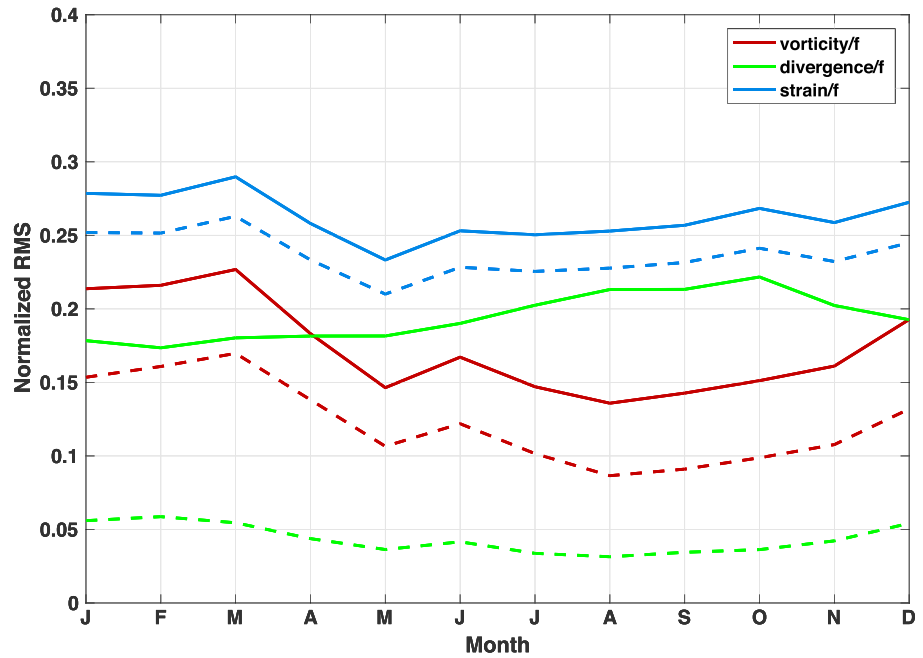
Figure 10. Monthly averages of normalized root-mean-square (RMS) vorticity (red), strain (blue), and divergence (green) estimated at the ocean surface. RMS is averaged over the subdomain shown in Figure 3 from one year of the (1/48)^\circ latitude-longitude cap 4320 model. RMS gradients are normalized by the local Coriolis parameter f . Solid/dashed lines are computed from hourly/daily averages, respectively.
