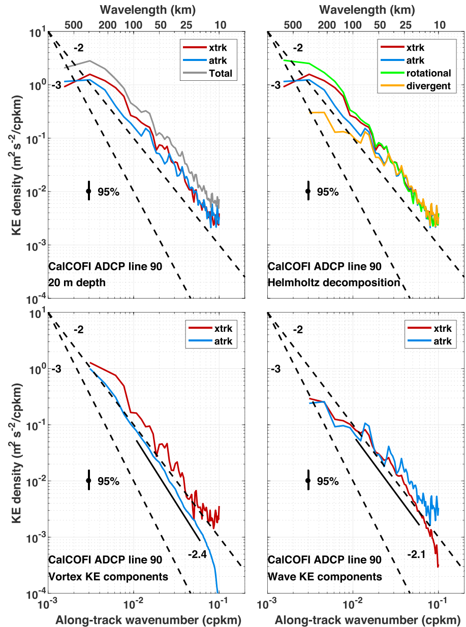
Figure 5. Helmholtz and wave-vortex decompositions of the acoustic Doppler current profiler (ADCP) kinetic energy (KE) spectra at 20-m depth for transects along line 90. (upper left) Across-track (red) and along-track (blue) KE components at 20-m depth for ADCP transects. Total (gray) ADCP KE as shown in Figure 4. (upper right) Across-track (red) and along-track (blue) KE components and the Helmholtz decomposition into rotational (green) and divergent (orange) components. (lower left) Vortex across-track (red) and along-track (blue) components. (lower right) Wave across-track (red) and along-track (blue) components. In all panels, black dashed lines show slopes of -2 and -3 for reference; 95% confidence limits are also shown. In the lower panels, the slope of the solid black line is a least squares fit to the KE estimates over the wavenumber range 0.01 to 0.06 cpkm, offset for clarity. CalCOFI = California Cooperative Oceanic Fisheries Investigations.
