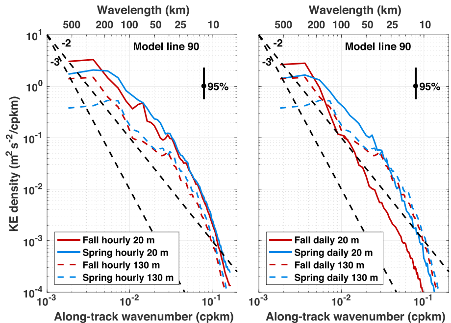
Figure 11. Seasonal kinetic energy (KE) spectra from the latitude-longitude cap 4320 model velocity estimates along line 90 for fall (red) and spring (blue). (left panel) KE estimates from hourly averages at depths of 20 (solid) and 130 m (dashed). (right panel) KE estimates from daily averages at depths of 20 (solid) and 130 m (dashed). Black dashed lines show slopes of -2 and -3 for reference.
