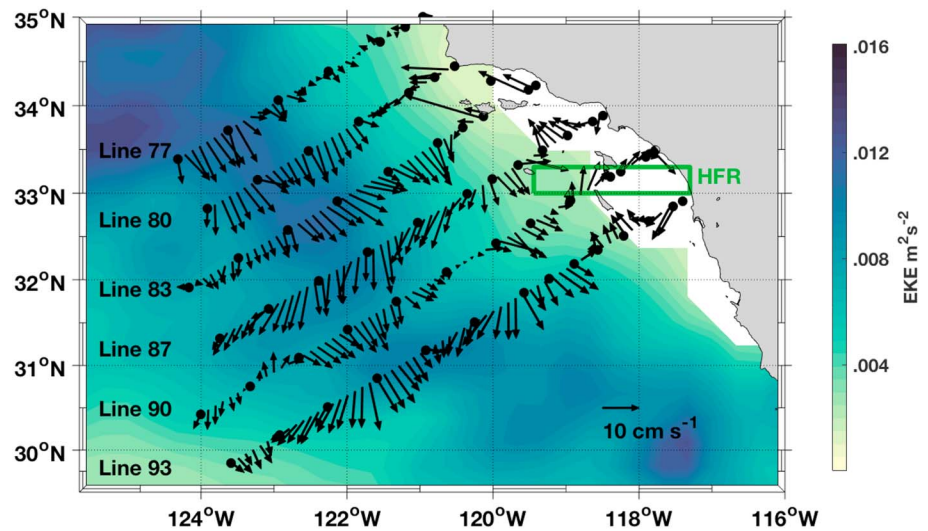
Figure 1. Mean (1993–2004) California Cooperative Oceanic Fisheries Investigations acoustic Doppler current profiler currents at 20-m depth superposed on eddy kinetic energy (EKE) estimated from Aviso altimetry for the same time interval. High-frequency radar (HFR) estimates were made by Kim et al. (2011) for the region denoted by the green box.
