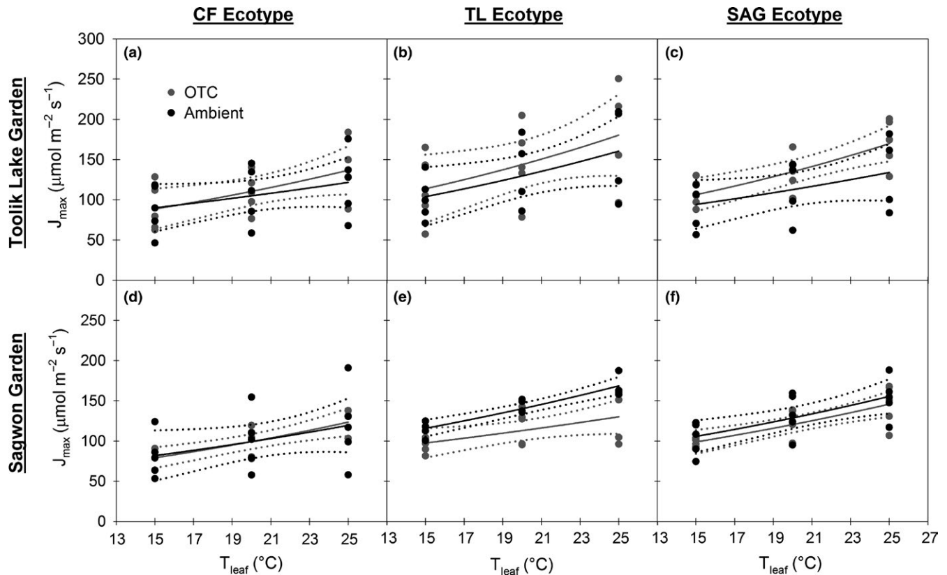
FIGURE 4 Maximum rate of electron transport ( J_{\text{max}} ) versus leaf temperature ( T_{\text{leaf}} ) for each ecotype of Eriophorum vaginatum (CF—Coldfoot, TL—Toolik Lake, SAG—Sagwon) within each garden (a–f). Each panel shows data and models for both the ambient (black) and open-top chamber (OTC) treatments (gray). Solid lines show the Arrhenius function used to model these relationships; dotted lines are 95% confidence intervals
