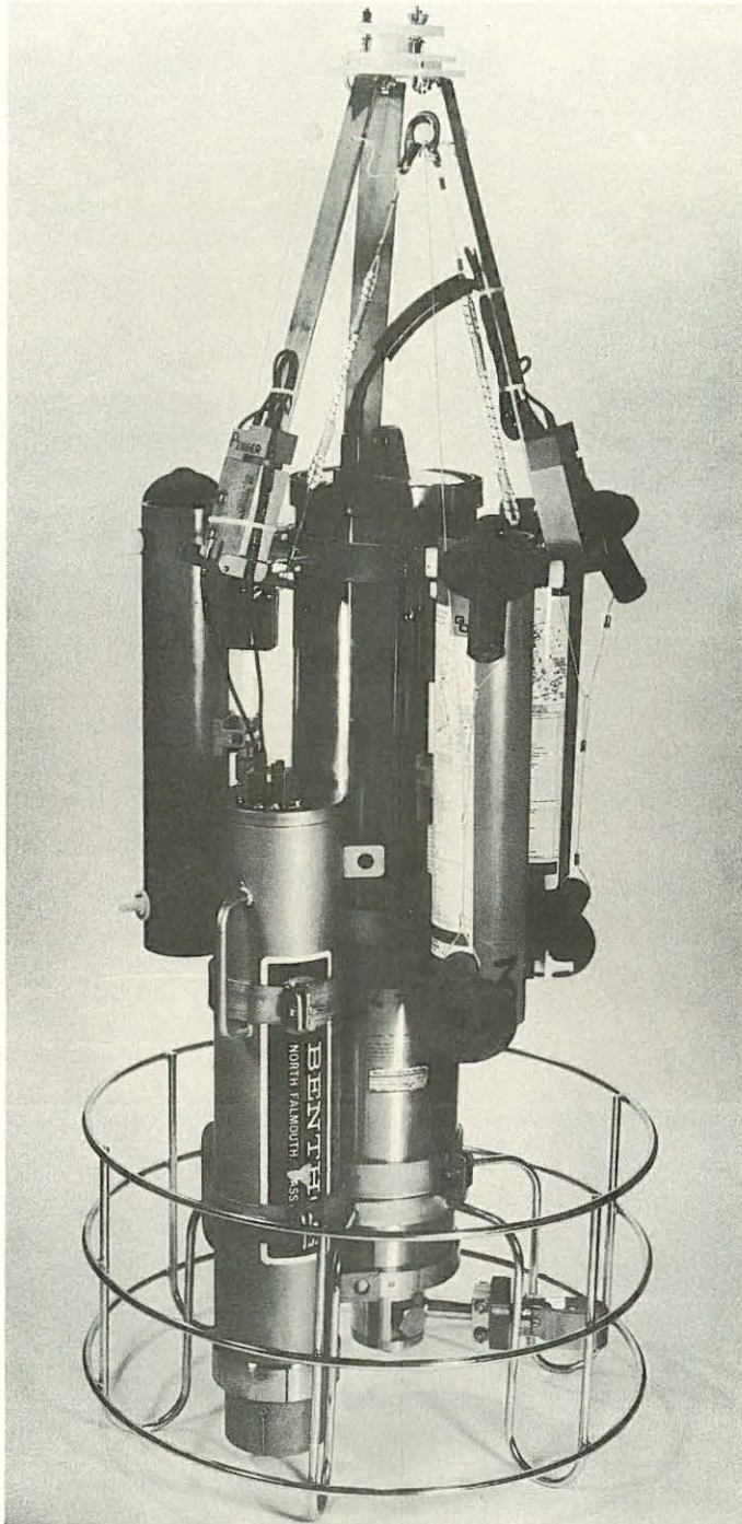
Figure 8. A photograph of the CTD/IR with the entire in situ calibration system mounted and ready for deployment.
