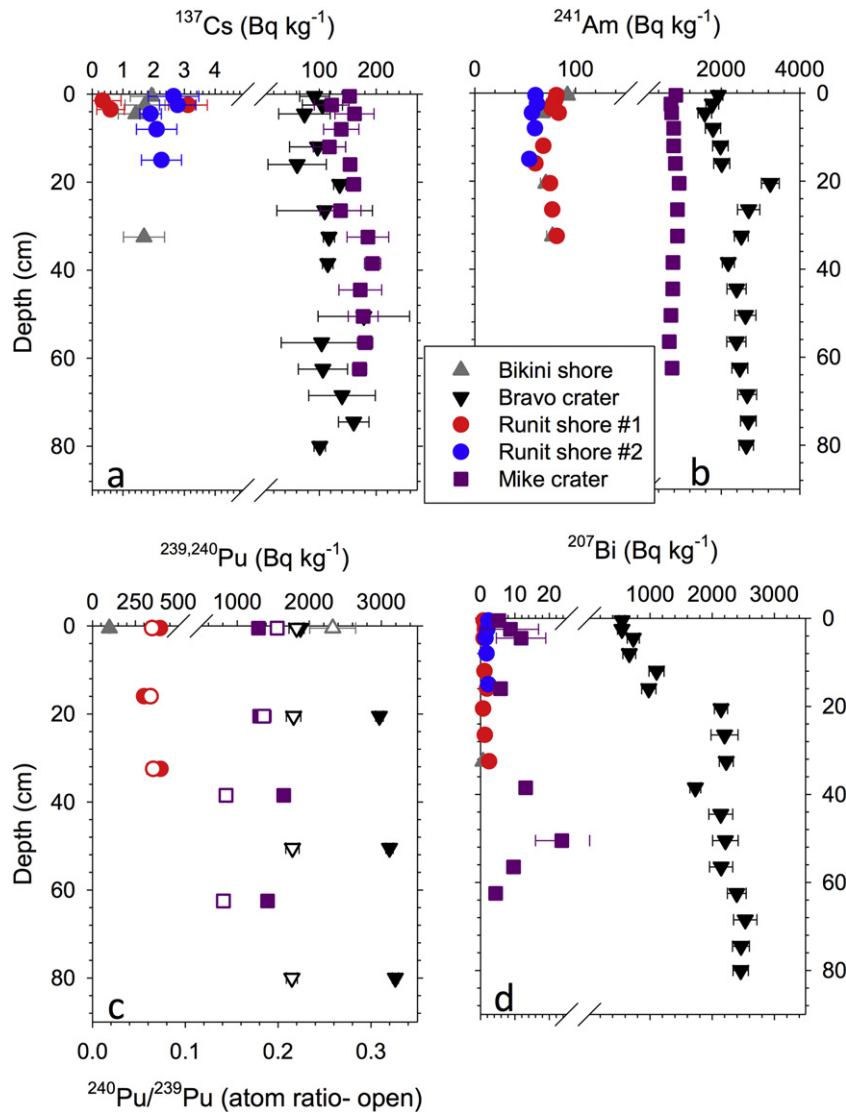
Fig. 5. Sediment core profiles vs. depth (cm- Y axis) for ^{137}\text{Cs} (a), ^{241}\text{Am} (b), ^{239,240}\text{Pu} (c) and ^{207}\text{Bi} (d). For each radionuclide the activities are along the upper x-axis in units of \text{Bq kg}^{-1} dry weight. For Pu, also shown are the ^{240}\text{Pu}/^{239}\text{Pu} atom ratios as open symbols with scale along the lower x-axis. Sample key is shown for Bikini shore (gray triangles), Bravo Crater (black inverted triangles), Runit shore (#1 and #2 are two sites, red and blue circles, respectively) and the Mike Crater (purple square). Error bars are shown if larger than the symbol size for each measurement. Data are in Table S2.
