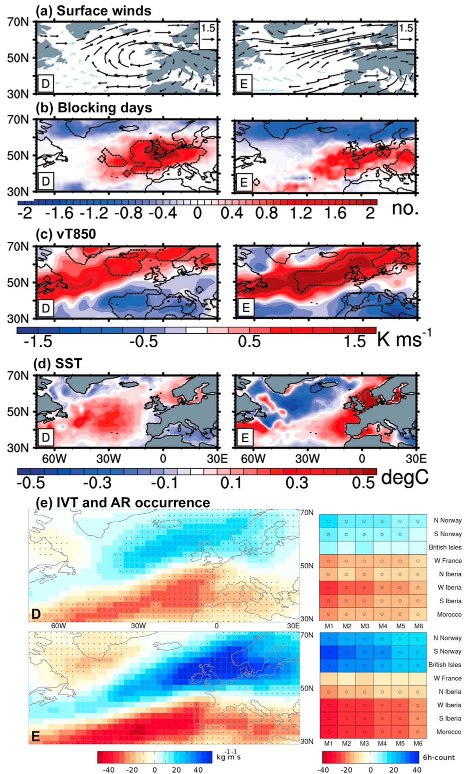
Figure 2. Composite anomalies of (a) surface winds (m/s), (b) number of blocking days per season, (c) 2–6 day band-pass filtered \langle v'T' \rangle at 850 hPa (K m/s), (d) SST (°C), and (e, f) integrated water vapor transport (IVT; kg/m/s) and atmospheric river (AR) occurrence, all for JFM for the period 1901–2010 for years in clusters D and E. Count of occurrence of AR events for eight target regions along the eastern Atlantic seaboard. Dashed contours and black vectors in Figures 2a–2d and stippling/circles in Figures 2e and 2f denote anomalies significant at the 2% significance level as estimated by Student’s t test. M1 to M6 represent the six method modifications of Brands et al. [2017] using different percentile thresholds to define an AR.
