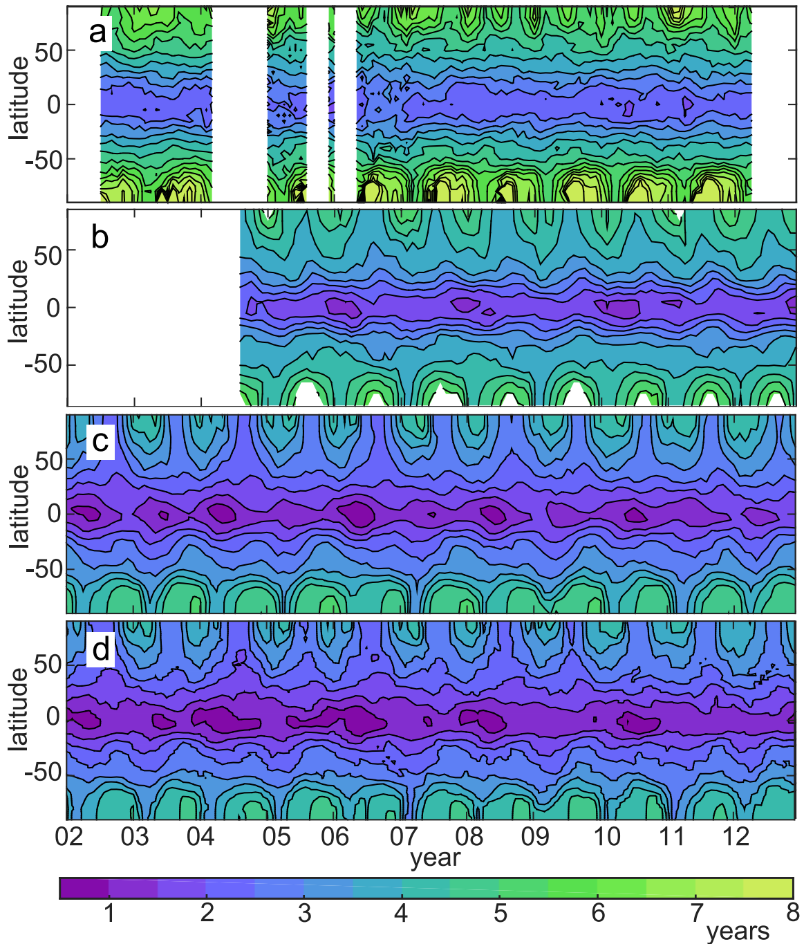
Figure 3-1: Age of air on the 500 K surface. (a) \text{SF}_6 from MIPAS, (b) \text{N}_2\text{O} from GOZ-CARDS, Andrews et al. 2001 (c) \text{SF}_6 from WACCM, and (d) WACCM ideal age tracer. Contours are every half year, and the ages in the Southern Hemisphere winter for MIPAS get above 8 years old.
