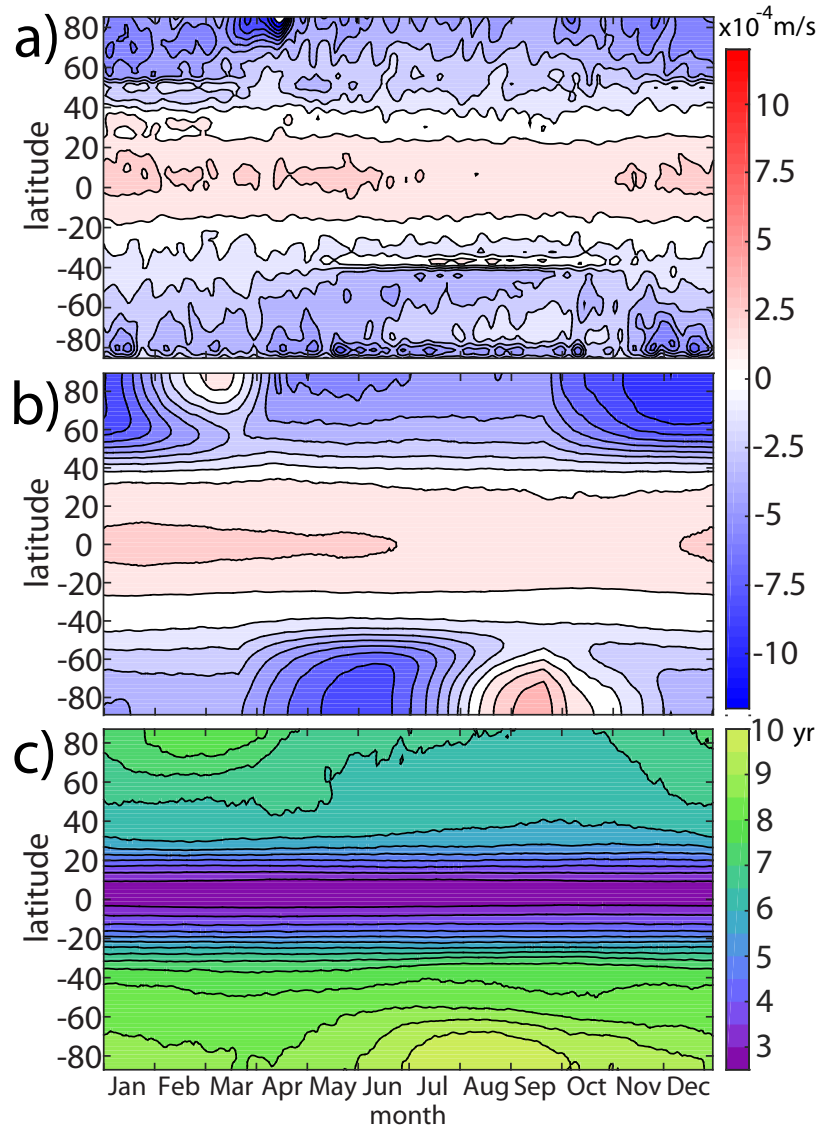
Figure 2-2: Annual cycle based on a 20 year average of the seasonally-varying model run for a) The residual circulation vertical velocity at 53 hPa. The field has been filtered using a binomial filter (14 days in time and 10^\circ in latitude) in order to smooth high temporal variability and cubed-sphere interpolation artifacts. b) The zonal mean diabatic vertical velocity at 500 K divided by the background stratification ( \dot{\theta}/\bar{\theta}_z ). The 500 K isentrope is on the annual average located near the 53 hPa surface. c) The age on the 500 K isentrope. Contour levels are 1.2 \times 10^{-4} m/s and 0.5 years.
