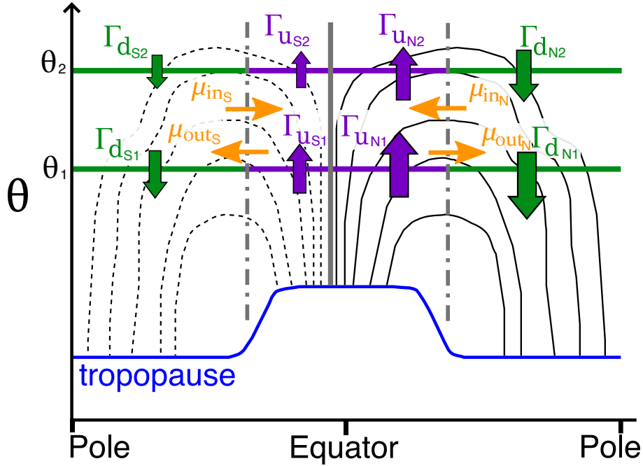
Figure 5-1: Schematic of the stratospheric circulation split into two “hemispheres” by a dynamical equator (dark gray solid line) corresponding to the zero streamline in the time mean of the circulation. Here the Northern Hemisphere is shown as having a greater meridional extent, consistent with reanalyses. Although this diagram shows the dynamical equator as vertical, in reality, it is tilted. Two separate isentropic levels are shown, with upwelling fluxes in purple and downwelling fluxes in green. The orange arrows are the mean entrainment and detrainment adiabatic mass fluxes between the extratropics and the tropics in each hemisphere. The black dotted and solid lines show the residual circulation streamlines. The dark gray dash-dot lines are the zero lines in the diabatic vertical velocity, \dot{\theta} , and like the dynamical equator, can have a varying latitude with height.
