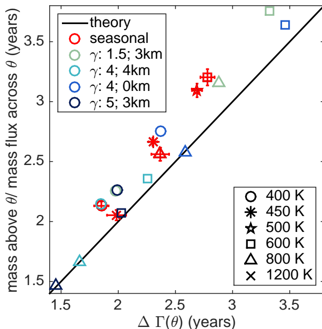
Figure 2-6: The ratio of mass above an isentrope to mass flux through an isentrope versus the difference between downwelling and upwelling age of air on the isentrope. The green and blue points are averages from the last 2000 days of perpetual-solstice runs as described in Table 2.1. The red points are the average of 50 annual averages from the seasonally-varying run with 4000 m topography and lapse rate of 4 K/km. The error bars are one standard deviation of the annual averages. The black line shows the one-to-one relationship predicted by the theory, and the different symbols are different isentropic levels.
