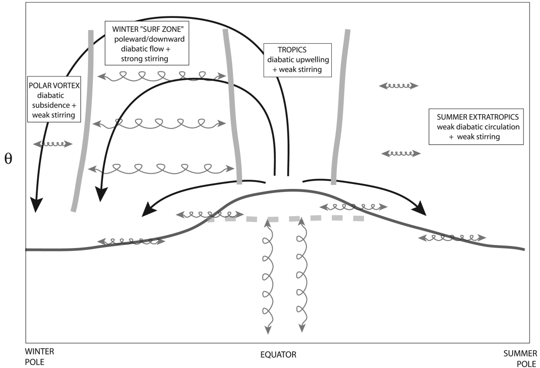
Figure 1-1: Schematic of stratospheric transport from Plumb 2007. The curve that extends across all latitudes is the tropopause and the black lines with arrows represent the meridional residual circulation. The grey bands are transport barriers, and the looped arrows represent along isentropic mixing. The vertical coordinate is \theta . See the text for a more detailed discussion
