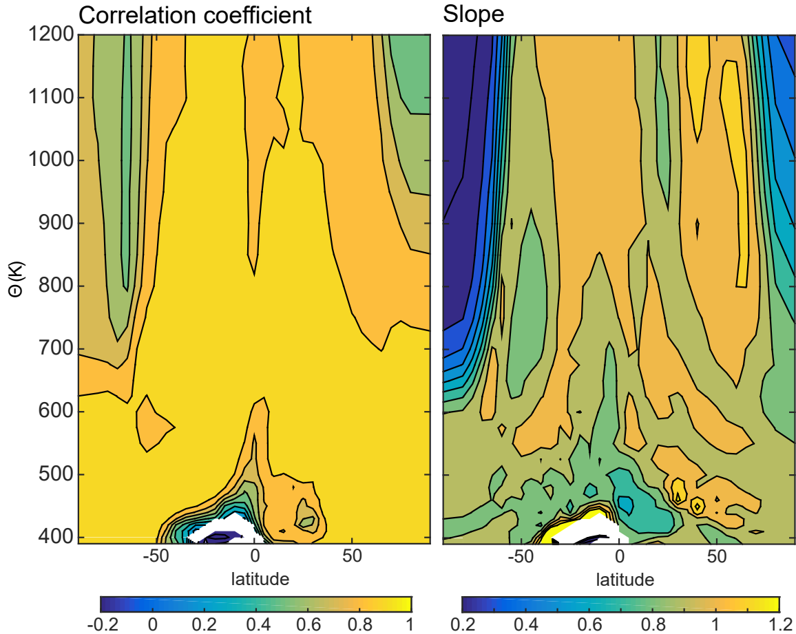
Figure 3-2: The zonal mean (a) correlation coefficient and (b) slope of correlation for the correlation between the time series of SF 6 -age and ideal age at every grid point for WACCM from 1990–2014.
