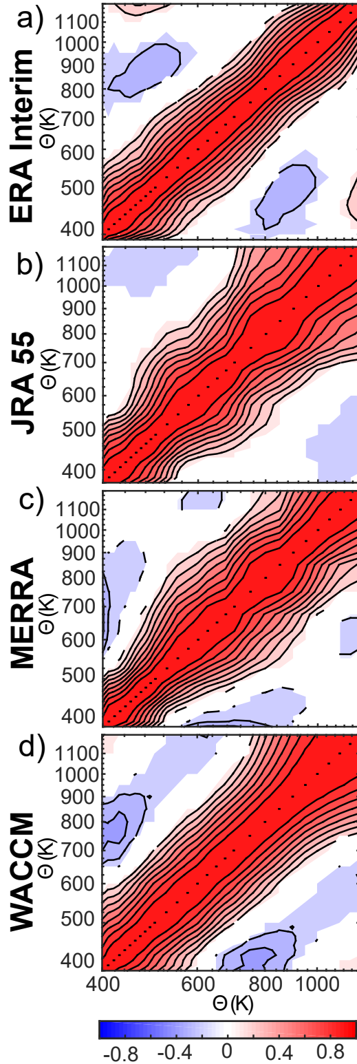
Figure 4-4: The spatial autocorrelation of the total diabatic overturning circulation strength from (a) ERA-Interim, (b) JRA55, (c) MERRA, and (d) WACCM. Correlations are only plotted where they are significant at the 95% confidence level, and the contour intervals are 0.1.
