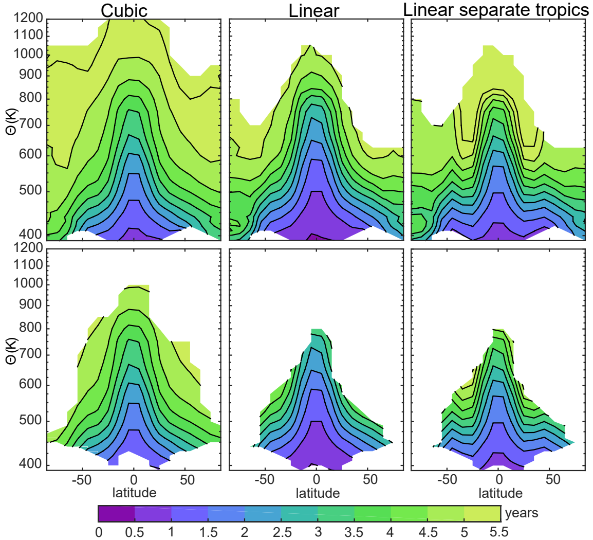
Figure 3-S8: The average age of air as a function of latitude and potential temperature based on GOZCARDS N 2 O data from 2007–2011 that has been converted to age of air using three different relationships: In the left column, the cubic relationship from Andrews et al. (2001) is used. In the middle column, the linear relationship determined by Strahan et al. (2011) is used. In the right column, the linear relationships shown above in Figure 3-S2 for the tropics and extratropics are used. MERRA pressure and temperature has been used to convert to isentropic surfaces. The first row is the mean value neglecting any data gaps, and the second row is the mean value only where there are no data gaps for the five years. Contours are every half year.
