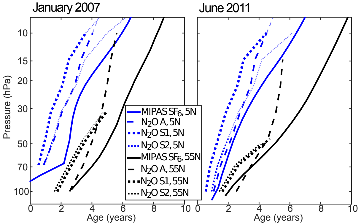
Figure 3-S5: Vertical profiles of age of air from MIPAS SF 6 and using three different empirical relationships for the relationship between N 2 O and age of air. The left panel is January 2007 and the right panel is June 2011. The blue lines show tropical profiles (5°N) and the black lines are extratropical or subpolar (55°N). Solid lines are MIPAS SF 6 -age, long dashed lines are derived from the cubic relationship between N 2 O and age of air from Andrews et al. (2001), bold dotted lines are derived from the linear relationship between N 2 O and age of air from Strahan et al. (2011), and the thin dotted lines are derived from the different tropical and extratropical linear fits between N 2 O and age shown in Figure 3-S2. Where the profiles are based on extrapolation of the fit to levels for which there was no data informing the fit, they are shown in light blue and gray and are thin.
