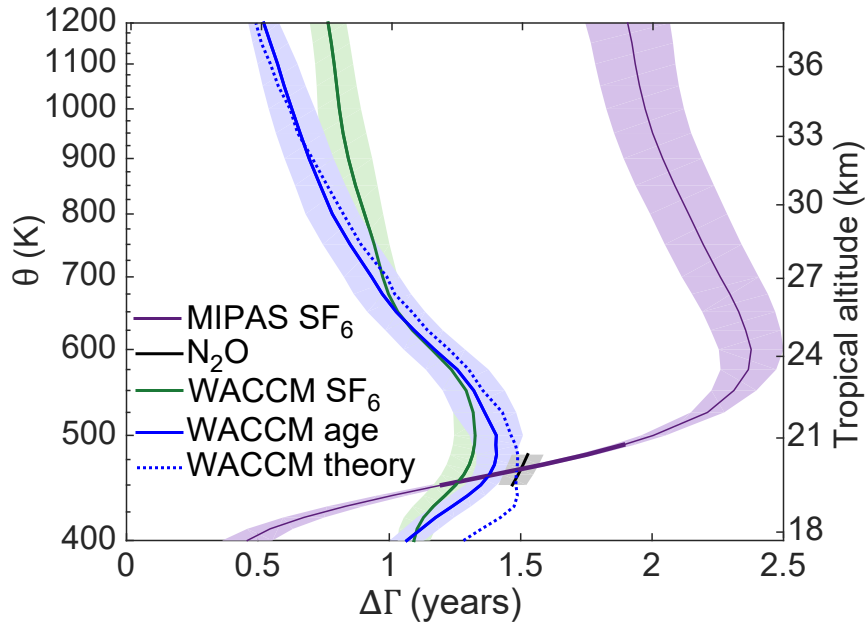
Figure 3-3: The average age difference between downwelling and upwelling age of air on each isentrope between 2007–2011. \Delta\Gamma is plotted in solid lines: MIPAS SF 6 -age in purple, GOZCARDS N 2 O age in black, WACCM SF 6 -age in green, and WACCM ideal age of air in the blue. The blue dotted line shows the ratio of the total mass above each isentrope to the mass flux through the isentrope ( M/\mathcal{M} ) from WACCM. The shading shows one standard deviation of the five annual averages that are averaged to get the mean. The mean height of each isentrope in the tropics (calculated from MIPAS pressure and temperature) is on the right y-axis. Where the line for the MIPAS SF 6 calculation is thick, there is confidence in both the data and in its conversion to age. Where it is thin, there are reasons to believe bias in either the data or in the conversion that lend less credence to its age difference.
