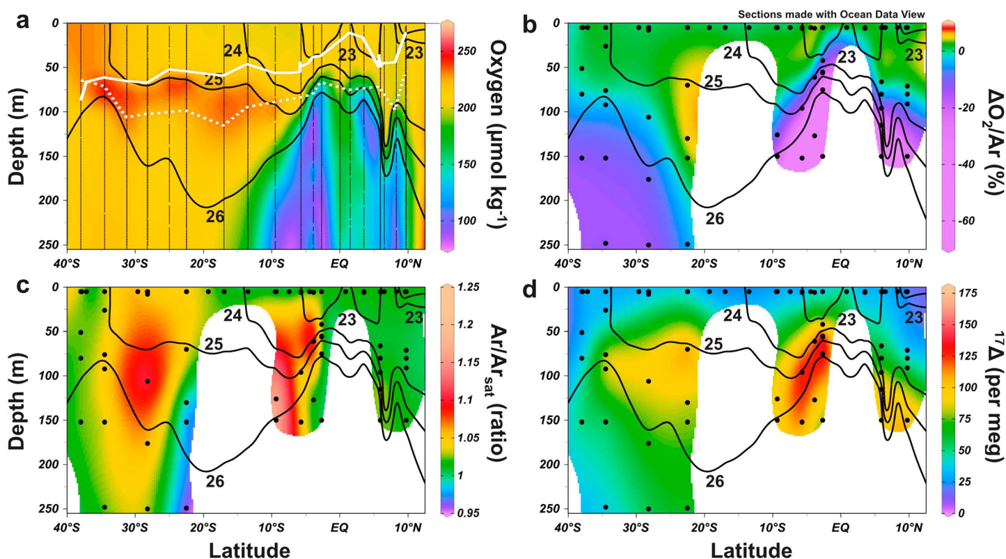
Figure 2. Meridional sections of (a) oxygen concentration, (b) biological oxygen saturation state \Delta O_2/Ar (supersaturation or undersaturation relative to atmospheric equilibrium), (c) argon saturation relative to atmospheric equilibrium Ar/Ar_{sat} and (d) the triple oxygen isotope tracer ^{17}\Delta (relative to the value of atmospheric oxygen). Sample locations are identified as black circles (except in Figure 2a where O_2 profiles from calibrated CTD are denoted by vertical lines), and labeled black contours are isopycnals of neutral density. Mean mixed layer depth (solid white line) and euphotic zone depth (dashed white line) at each location are also plotted in Figure 2a. Sections are gridded with horizontal and vertical length scales of 1^\circ latitude and 20 m depth using Data-Interpolating Variational Analysis in Ocean Data View [Schlitzer, 2015; http://odv.awi.de ]. Tracer values from the first sample location along the transect ( 37.1^\circ S , 49.9^\circ W ) are not plotted so that latitude increases monotonically along the section.
