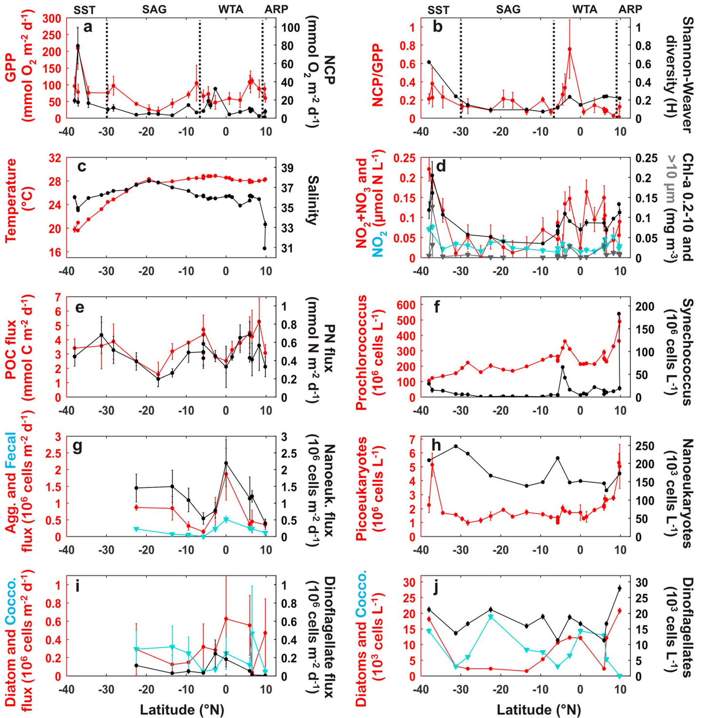
Figure 3. Measured and calculated parameters plotted against latitude. Biogeographic provinces are noted with dashed lines and abbreviations as in Figure 1. Throughout, the first variable on the left axis is marked by red filled circles and the second marked by cyan triangles, and the first variable on the right axis is marked by black circles and the second by gray triangles (axis labels colored similarly). Top row: (a) gross primary production (GPP) and net community production (NCP); and (b) the NCP/GPP ratio and Shannon-Weaver diversity ( H ) phytoplankton community. Second row: (c) temperature and salinity; and (d) total nitrite plus nitrate, nitrite only, and chlorophyll a concentrations for the 0.2–10 \mu\text{m} and >10 \mu\text{m} size fractions. Left-hand column from third row down: particle fluxes at 125 m, including (e) particulate organic carbon (POC) and particulate nitrogen (PN) fluxes; (g) cell aggregate, fecal pellet, and nanoeukaryote number fluxes; and (i) diatom, coccolithophore, and dinoflagellate number fluxes. Right hand column from third row down: abundances of (f) Prochlorococcus and Synechococcus ; (h) picoeukaryotes and nanoeukaryotes, and (j) diatoms, coccolithophores, and dinoflagellates. Standard deviations are plotted as error bars (or are smaller than the marker size) on all variables except Shannon-Weaver diversity ( H ), which is a lower bound (see section 3.3 and Table S3).
