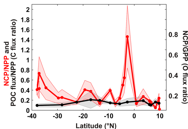
Figure 5. Export ratio estimates from O_2/Ar -based net community production (NCP) and particulate organic carbon (POC) flux, relative to net primary production (NPP; scaled from triple oxygen isotope based gross primary production, GPP). NCP/NPP export ratio and standard deviation (red), and the POC flux/NPP export ratio and standard deviation (black) are plotted in carbon units on the left-hand axis and oxygen units (relative to GPP rather than NPP) on the right-hand axis. NCP/NPP peaks at 37.2^\circ S and 2.9^\circ S are discussed in the text.
