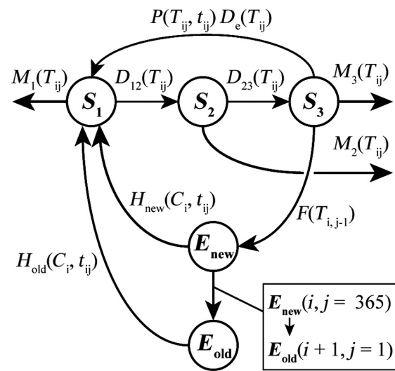
Fig. 3. Flow model describing the stage-structured Bythotrephes ’ population model. The active population in the water column ( S_1 – S_3 ) and resting egg bank in sediment ( E_{\text{old}} , E_{\text{new}} ) are stages (depicted as circles) in the model governed by temperature-dependent ( T or C in the case of time since a thermal cue) and time ( t )-dependent processes (depicted as arrows): development ( D ), reproduction ( P , asexual, and F , sexual), mortality ( M ), and hatching from the egg bank ( H ).
