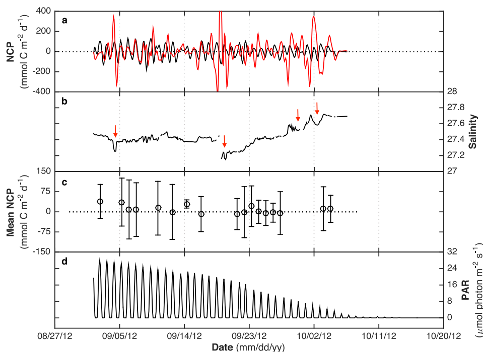
Figure 5. (top) NCP from the bandpass filtered DIC (red) and DO (black) ITP-64 data. DIC NCP was multiplied by -1 to make NCP positive during periods of net photosynthesis. Abrupt changes in salinity (highlighted by downward arrows) indicate potential advection of waters with different levels of p\text{CO}_2 and DO. Daily mean (open circle) \pm standard deviation of NCP based on DO is shown in the third plot. The mean was calculated over a 24 h period starting at 8 A.M. local time with the periods omitted when salinity was significantly changing. The PAR data were calculated from the incident solar radiation that was initially scaled using the surface PAR data collected on the ship (see Methods).
