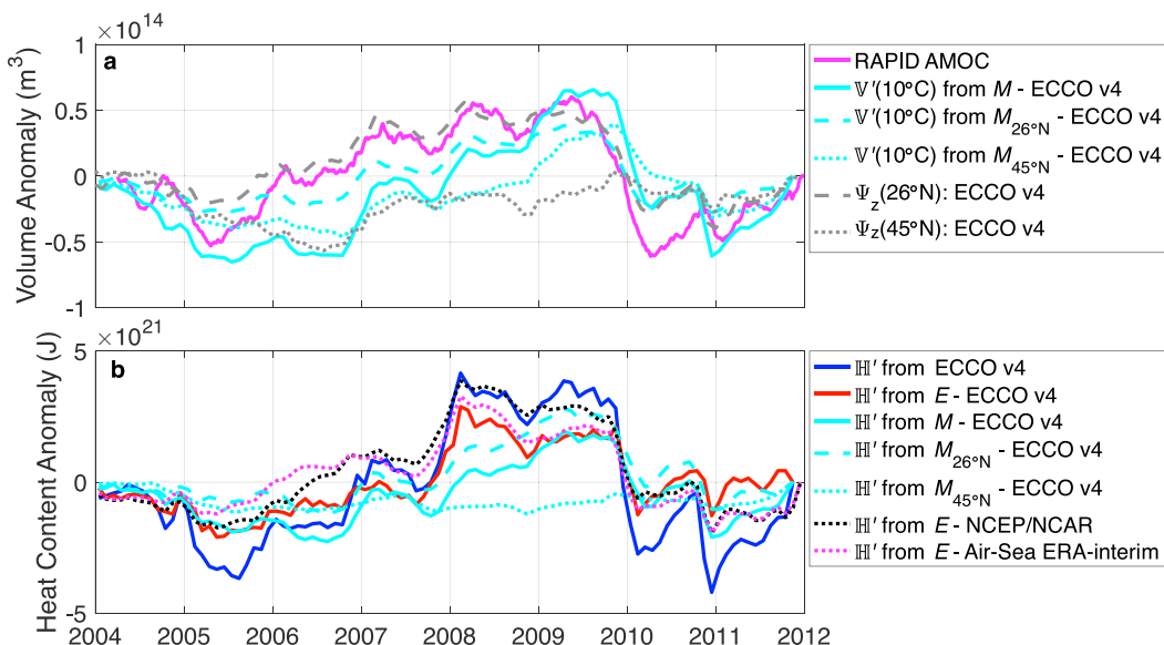
FIG. 7. (a) AMOC monthly mean anomaly (2004–12), estimated from RAPID–WATCH (magenta). Volume anomaly [ \Psi' ; Eq. (7)] for temperatures greater than 10^\circ\text{C} calculated using M (cyan): M_{26^\circ\text{N}} (cyan dashed) and M_{45^\circ\text{N}} (cyan dotted). Time-integrated AMOC monthly mean anomaly (2004–12) from ECCO v4 (i.e., \Psi_z ) at 26^\circ and 45^\circ\text{N} (dashed and dotted gray lines respectively). (b) Implied heat content anomaly [ \mathbb{H}' from Eq. (8)] at \Theta > 10^\circ\text{C} from the monthly dV/dt from ECCO v4 (blue), E from ECCO v4 (red), M from ECCO v4 (cyan), M_{26^\circ\text{N}} from ECCO v4 (cyan dashed), M_{45^\circ\text{N}} from ECCO v4 (cyan dotted), E from NCEP–NCAR (black dotted), and E from ERA–Interim (magenta dotted).
