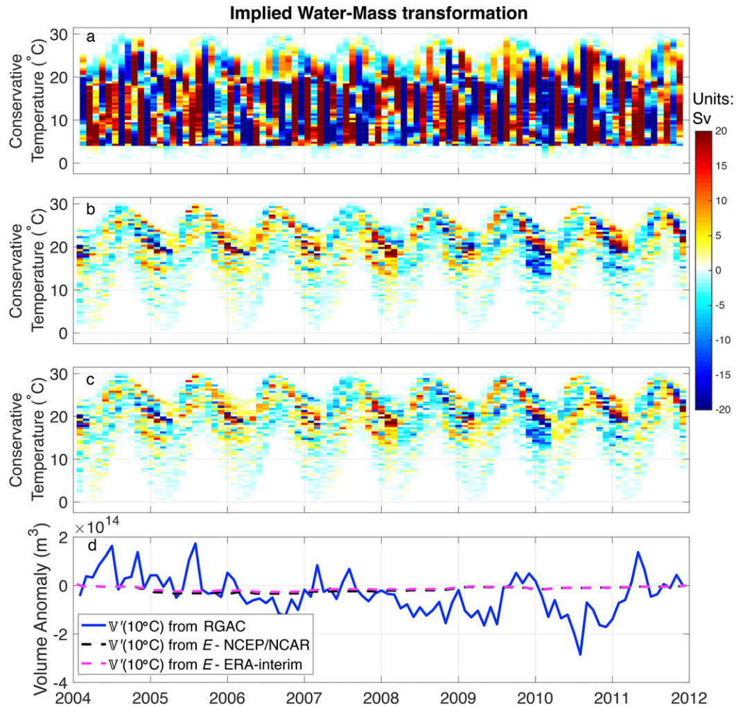
FIG. 5. (a) Total monthly dV/dt [see Eq. (4)] from RGAC between 26^{\circ} and 45^{\circ}\text{N} . The mean (2004–2012) seasonal cycle has been removed. (b) Monthly diathermal transformation due to air–sea heat fluxes [ E ; Eq. (6)] from NCEP–NCAR air–sea heat fluxes using Reynolds SST between 26^{\circ} and 45^{\circ}\text{N} . The mean (2004–12) seasonal cycle has been removed. (c) As in (b), but using ERA-Interim air–sea heat fluxes. (d) Volume anomaly [ V' ; Eq. (7); m 3 ] for temperatures greater than 10^{\circ}\text{C} .
