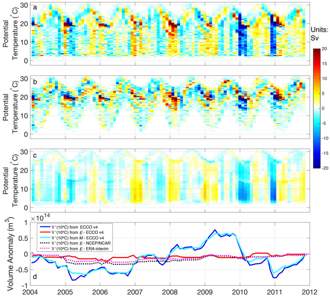
FIG. 6. (a) Total monthly dV/dt [see Eq. (4)] from ECCO v4 between 26^{\circ} and 45^{\circ}\text{N} . The mean (2004–2012) seasonal cycle has been removed. (b) Monthly diathermal transformation due to air–sea heat fluxes [ E ; Eq. (6)] from ECCO v4 between 26^{\circ} and 45^{\circ}\text{N} . The mean (2004–12) seasonal cycle has been removed. (c) Transformation implied by the volume change per \Theta class due to monthly variations in the transport per \Theta class at 26^{\circ}\text{N} minus the volume change per \Theta class due to monthly variations in the transport at 45^{\circ}\text{N} , from ECCO v4 [i.e., M from Eq. (4)]. The mean (2004–12) seasonal cycle has been removed. (d) Volume anomaly [ V' ; Eq. (7); \text{m}^3 ] for temperatures greater than 10^{\circ}\text{C} .
