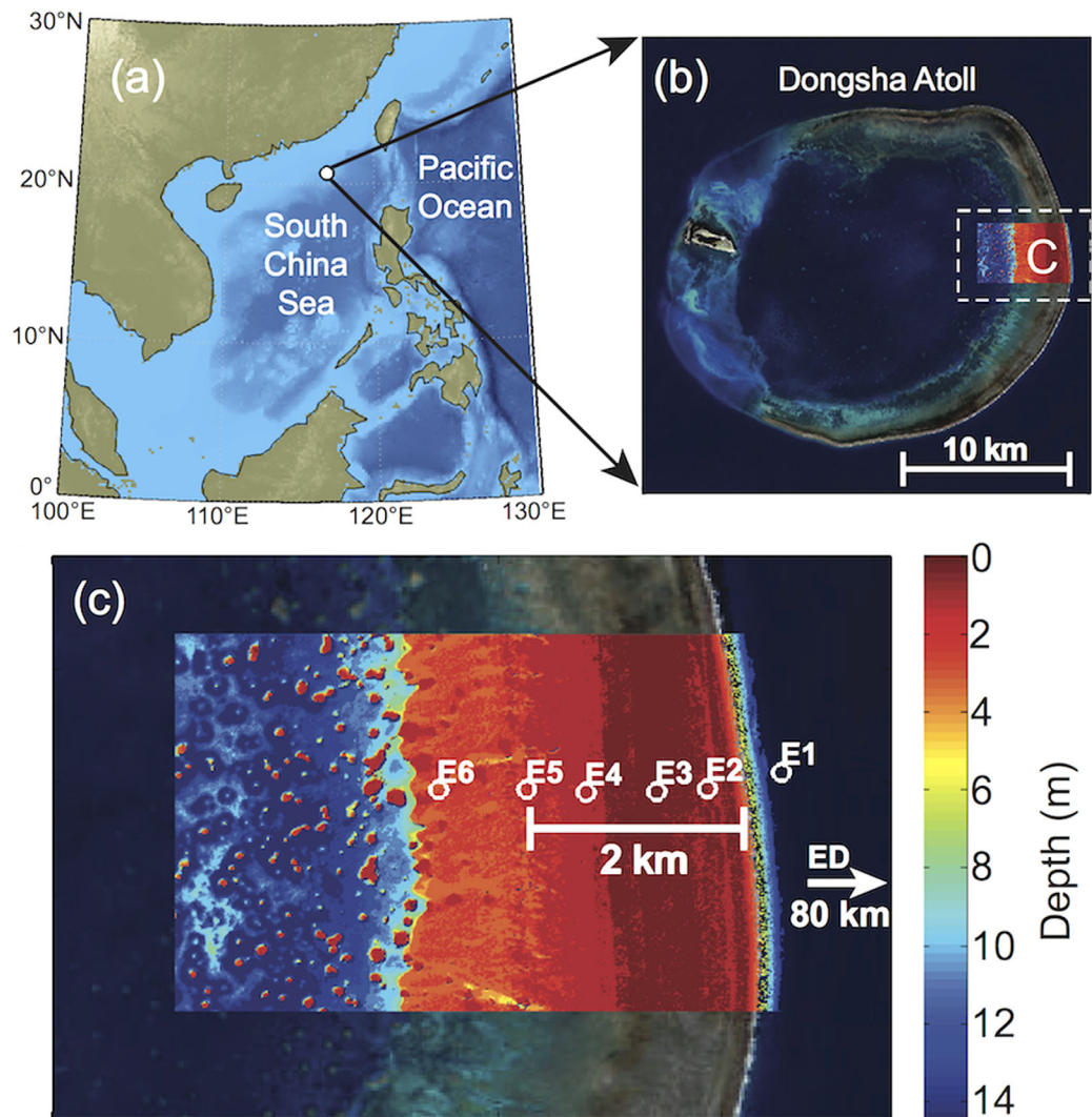
Figure 1. Map of Dongsha Atoll in the northern South China Sea. (a) Regional map, (b) satellite image of Dongsha Atoll from the Taiwan National Space Organization, and (c) study location and sampling stations on the eastern margin of the atoll. In Figure 1c, bathymetry data from Shih et al. [2011] are overlaid on the satellite imagery. Offshore samples were collected at station ED, located 80 km east of the atoll, and fore reef samples were collected at station E1. Instruments were deployed across the reef flat (Table 1), but the primary location for reef-water sampling was E5, located 2 km west of the reef crest.
