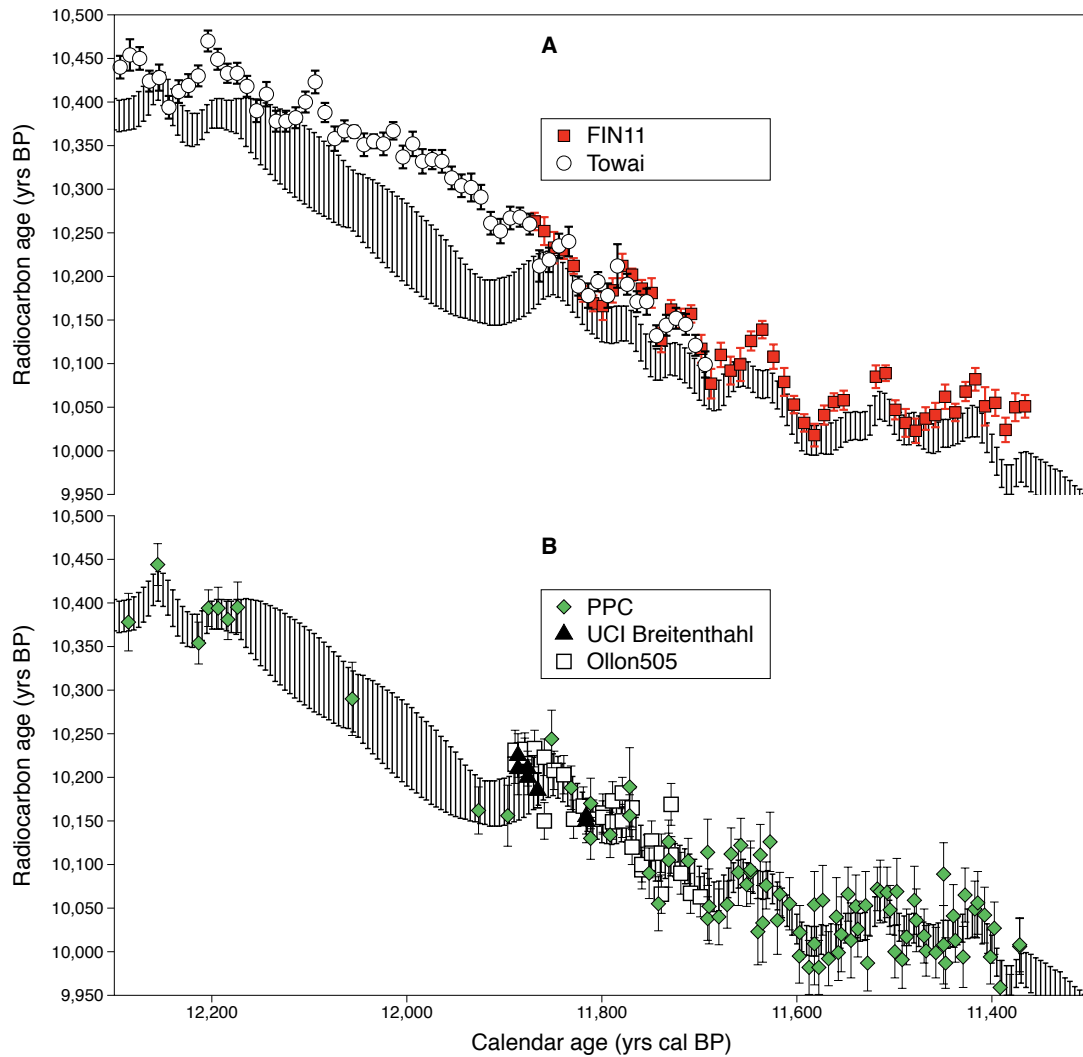
Figure 2. A: Floating SH Towai and FIN11 datasets. 2B: NH datasets. (i) Known calendar-age: Preboreal pine chronology (PPC) and Breitenhahl (UCI); (ii) Floating: Ollon505 (new Wk and HD data; Hogg et al. 2013a). IntCal13 curve (black 1\sigma error bars) given in both plots.
