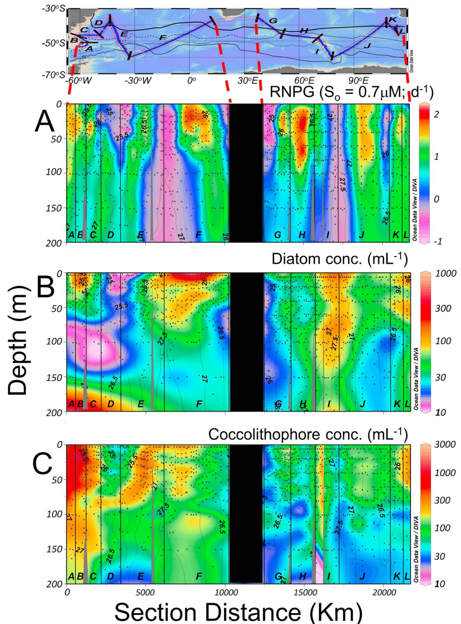
Figure 3. Vertical sections from Melville no. 1101 and Revelle no. 1202 cruises. The top inset shows the cruise track with letters designating sections of the cruise track. (a) Sections of RNPg ( d^{-1} ) where positive values are regions where nonsiliceous phytoplankton growth would be expected to be favored, while negative values represent regions and depths where potential diatom growth would be expected. (b) Diatom abundance ( mL^{-1} ) as determined with the FlowCAM. (c) Sections of coccolithophore concentration ( mL^{-1} ) as determined with polarized light microscopy. In all plots, vertical lines and letters designate the sections shown in inset. Frontal climatologies are indicated in top inset with different line patterns (from north to south): thick solid line = Subtropical Front, dashed line = Subantarctic Front, fine dash = Polar Front, thin solid line = ACC boundary [Orsi et al. , 1995]. Density isopleths overlaid onto Figures 3a–3c.
