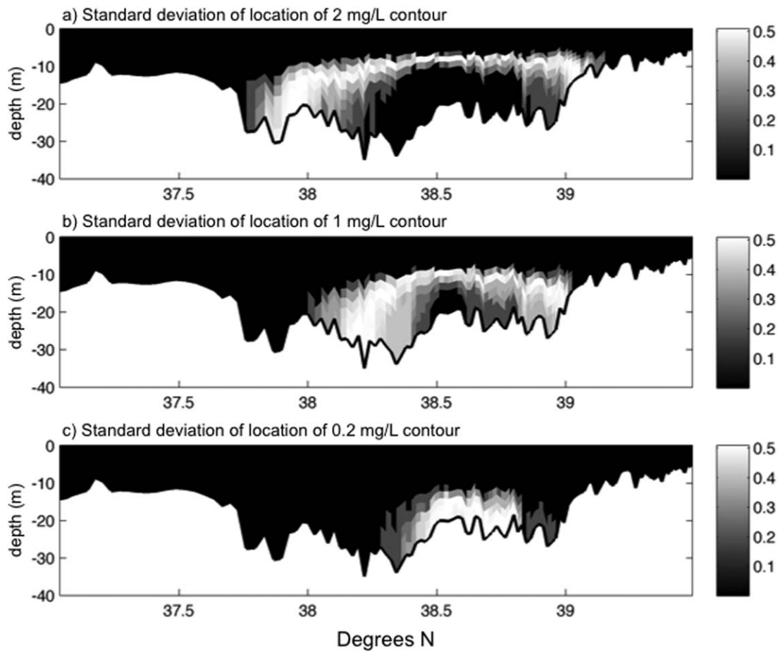
Fig. 12. Standard deviation of the location of the summer (June–August). (a) 2 \text{ mg L}^{-1} thalweg DO contour; (b) 1 \text{ mg L}^{-1} thalweg DO contour; (c) 0.2 \text{ mg L}^{-1} thalweg DO contour.
