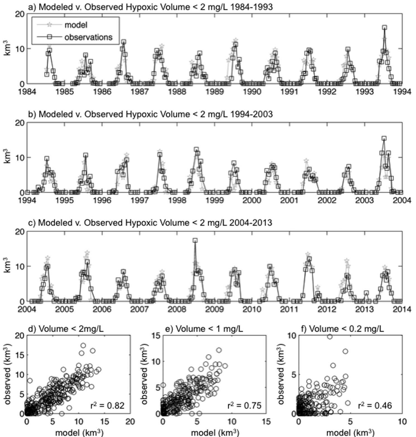
Fig. 3. Comparison of the predicted hypoxic volume < 2 mg L -1 (gray stars) to the observed (black squares) volume based on individual CBP cruises for (a) 1984–1993, (b) 1994–2003, and (c) 2004–2013. Scatter plots comparing the model prediction and observed hypoxic volumes for (d) < 2 mg L -1 threshold, (e) < 1 mg L -1 threshold, and (f) < 0.2 mg L -1 threshold. Reported correlations are all significant at p < 0.05 .
