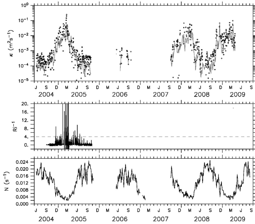
Fig. 8. Top panel shows on a log scale 5-day smoothed diffusivity ( \kappa ) at the base of the mixed layer (plus marks) and their errors (grey line). Values below the grey line can be considered noise. Middle panel shows hourly values of 1/Ri on a linear scale. A nominal critical Ri is shown as a grey dashed line. The bottom panel shows the 5-day smoothed buoyancy frequency ( N ) on a linear scale.
