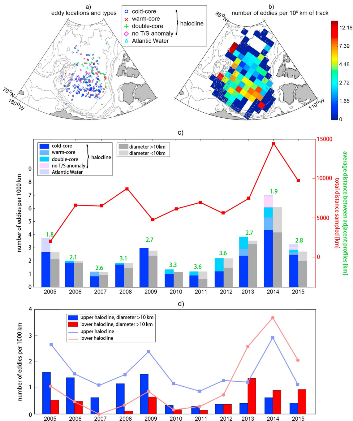
Figure 2. (a) Eddy locations and types sampled between 2005 and 2015 from all ITPs. (b) Number of eddies per 10 6 km of ITP drift track in each 100 km × 100 km cell. (c) Time series of the number of anticyclonic eddies per 1000 km (bars) and total cumulative (along track) distance (red line) sampled from 2005 to 2015. Green numbers indicate the average distance (km) between adjacent ITP profiles (i.e., average horizontal resolution). Colored bars include all types of anticyclonic eddies. Grey bars include only halocline anticyclonic eddies detected based on temperature and salinity fields and not velocity. (d) Time series of the number of upper halocline eddies (blue, core salinity <32) and the number of lower halocline eddies (red, core salinity >32) per 1000 km. The lines include all halocline anticyclonic eddies identified only from temperature and salinity measurements, and the bars include only eddies larger than 10 km in diameter.
