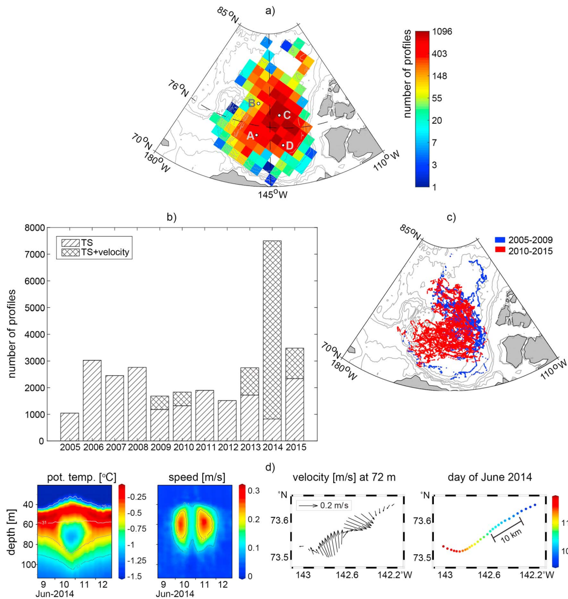
Figure 1. (a) Number of profiles used in this analysis per 100 km × 100 km cell in the Canada Basin between 2005 and 2015 from all ITPs. The locations of the four BGEF moorings (A, B, C, and D) are also indicated. Dashed lines divide the basin into four sectors corresponding to each of the four moorings. (b) Number of profiles with measurements from ITP-Vs (including horizontal velocity in addition to temperature and salinity) and ITPs (only temperature and salinity) in each year. (c) The locations of all ITP measurements from 2005 to 2009 (blue) and 2010 to 2015 (red). (d) A typical upper halocline eddy (core salinity <32, sampled by ITP 77 in 2014 in the southern portion of the basin). First panel: potential temperature (°C)-depth (m) section overlaid with salinity contours; second and third panels: velocity magnitude (m/s)-depth (m) section and the velocity field at the eddy core depth; fourth panel: ITP drift track through the eddy showing dates and horizontal scale.
