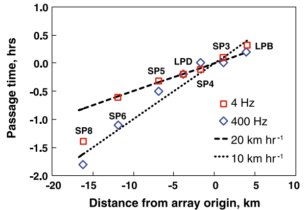
FIG. 13. The passage time for the 400-Hz pressure spectrum (blue diamonds) indicates a front speed close to 10 km h -1 . This hinges on the large difference between the passage time estimated from 4 Hz (red squares) and 400 Hz for station SP6 at -12 km. For this plot, the 400-Hz passage times in Table 4 have been shifted by 8.1 h, so the time is 0 at the array origin.
