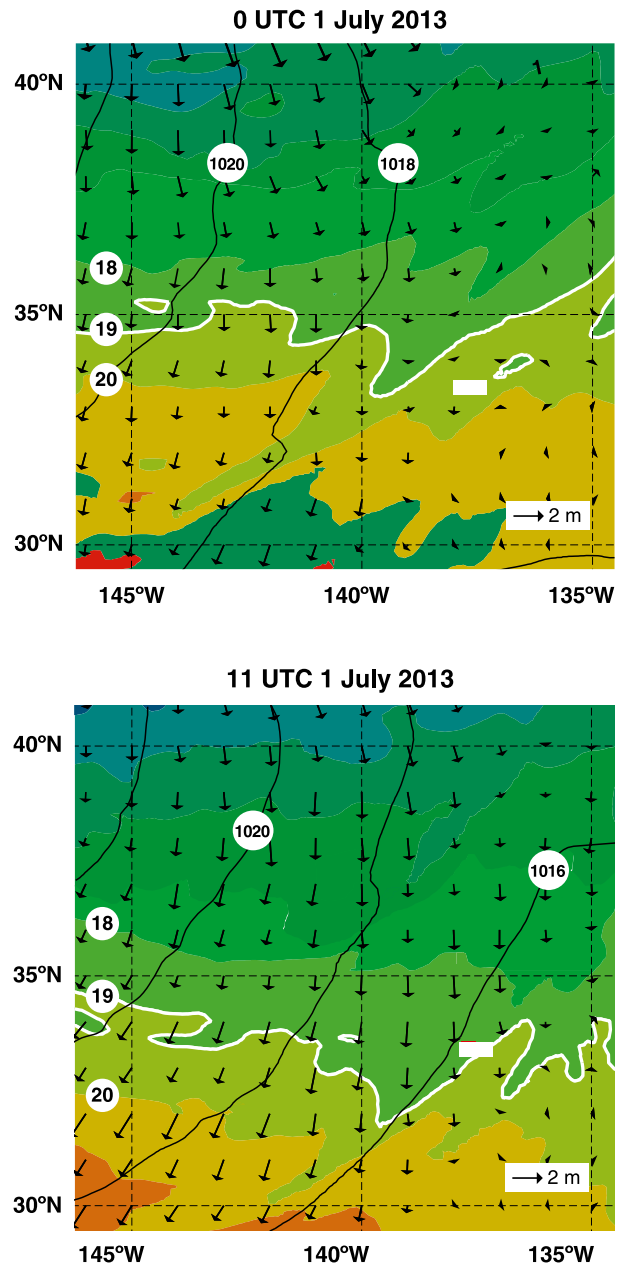
FIG. 5. The passage of the front over OBSANP is clear in the southerly migration of the 2-m temperature (color), as well as the increase in the wind-sea significant wave height (black vectors). The surface pressure (black contours) is less diagnostic. The color shading for the 2-m temperature has 1° steps. The wind-sea arrows are plotted every 1°, much coarser than the 28-km resolution of the model. The white rectangle shows the OBSANP location and is drawn to scale (see Fig. 1). These charts are about 1000 km on a side.
