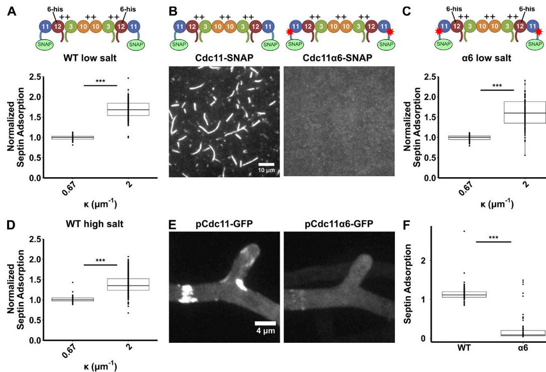
Figure 4. Curvature preference remains intact in single complexes, but filament formation is required for stable membrane association. (A) Adsorption of 25 nM 6xHIS WT Cdc11–SNAP488 complexes to 1-µm ( \kappa = 2 \mu\text{m}^{-1} ) and 3-µm ( \kappa = 0.67 \mu\text{m}^{-1} ) beads coated in 2% DGS-Ni 2+ NTA lipids in 100 mM KCl. For visualization of fold enrichment, data were normalized to 3-µm beads. (B) WT Cdc11–SNAP complexes and Cdc11- \alpha 6 -SNAP complexes, containing point mutations in the polymerization interface of Cdc11, were diluted to 250 nM in 50 mM KCl to promote filament formation and visualized on a polyethylene glycol-coated coverslip. (C) Adsorption of 100 nM 6xHIS Cdc11- \alpha 6 -SNAP488 complexes to 1-µm ( \kappa = 2 \mu\text{m}^{-1} ) and 3-µm ( \kappa = 0.67 \mu\text{m}^{-1} ) beads coated in 2% DGS-Ni 2+ NTA lipids in 100 mM KCl. (D) Adsorption of 25 nM 6xHIS WT Cdc11–SNAP488 complexes to 1-µm ( \kappa = 2 \mu\text{m}^{-1} ) and 3-µm ( \kappa = 0.67 \mu\text{m}^{-1} ) beads coated in 2% DGS-Ni 2+ NTA lipids in 300 mM KCl. (E) WT and \alpha 6 mutant Cdc11-GFP expressed and imaged in live A. gossypii . (F) Membrane adsorption of 100 nM WT and Cdc11- \alpha 6 -SNAP488 complexes on anionic-supported lipid bilayer (25% PC, 75% PI, and trace RhPE)-coated 1-µm beads. In A, C, D, and F, n \geq 43 for each size. Dunn test results: ***, P < 0.005 .
