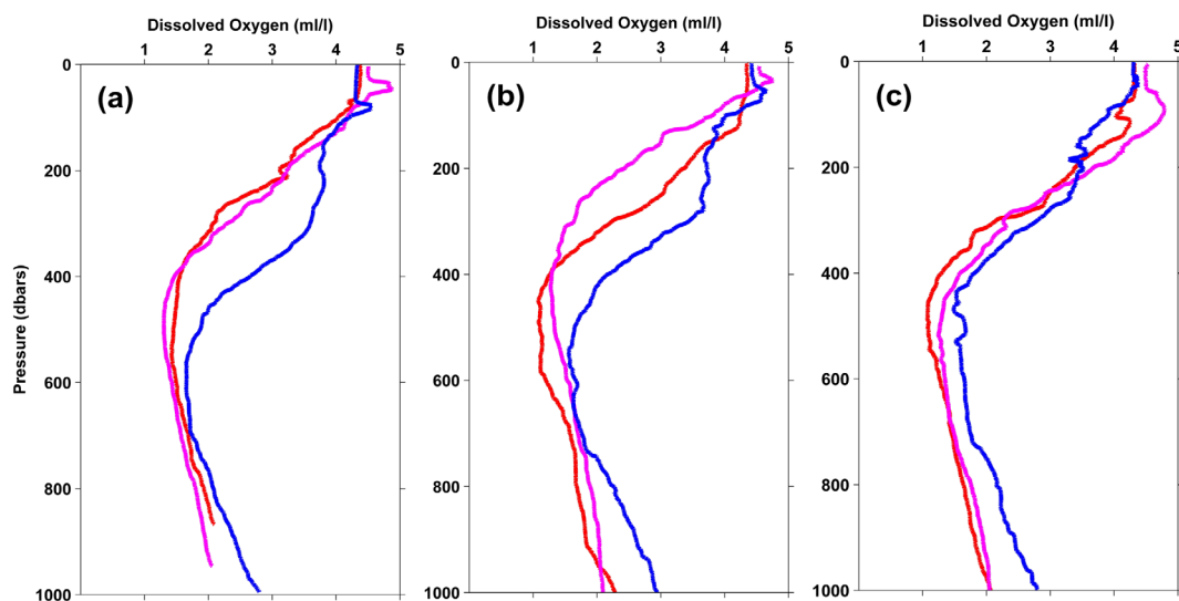
Figure 5. Dissolved oxygen profiles for the stations (a) NRS5, (b) NRS4, and (c) NRS3 obtained in March 2010 (red), October 2011 (magenta), and November 2012 (blue).
