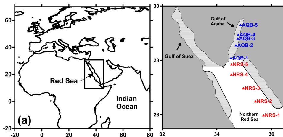
Figure 1. The location of the Red Sea, the line of hydrographic stations repeatedly carried out in November 2013 and March 2015, and the areas of spatially averaged MODIS SST (shaded). Stations NRS-4, NRS-3, and NRS-2 coincide with stations carried out during KAUST 2010 and 2011, and KFUPM 2012 expeditions.
