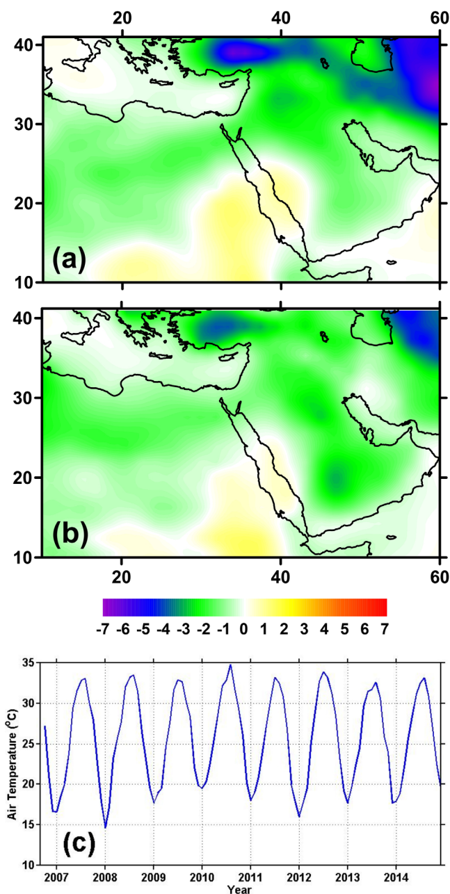
Figure 7. Mean winter (DJF) air temperature anomaly (°C) for (a) 2008 and (b) 2012 and (c) monthly mean air temperature from Eilat meteo station.
