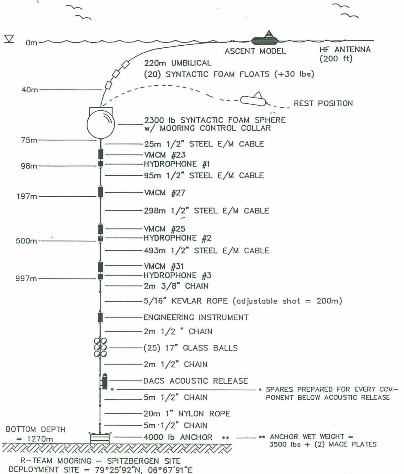
FIGURE 6 DESIGN AS SET (1270m)
