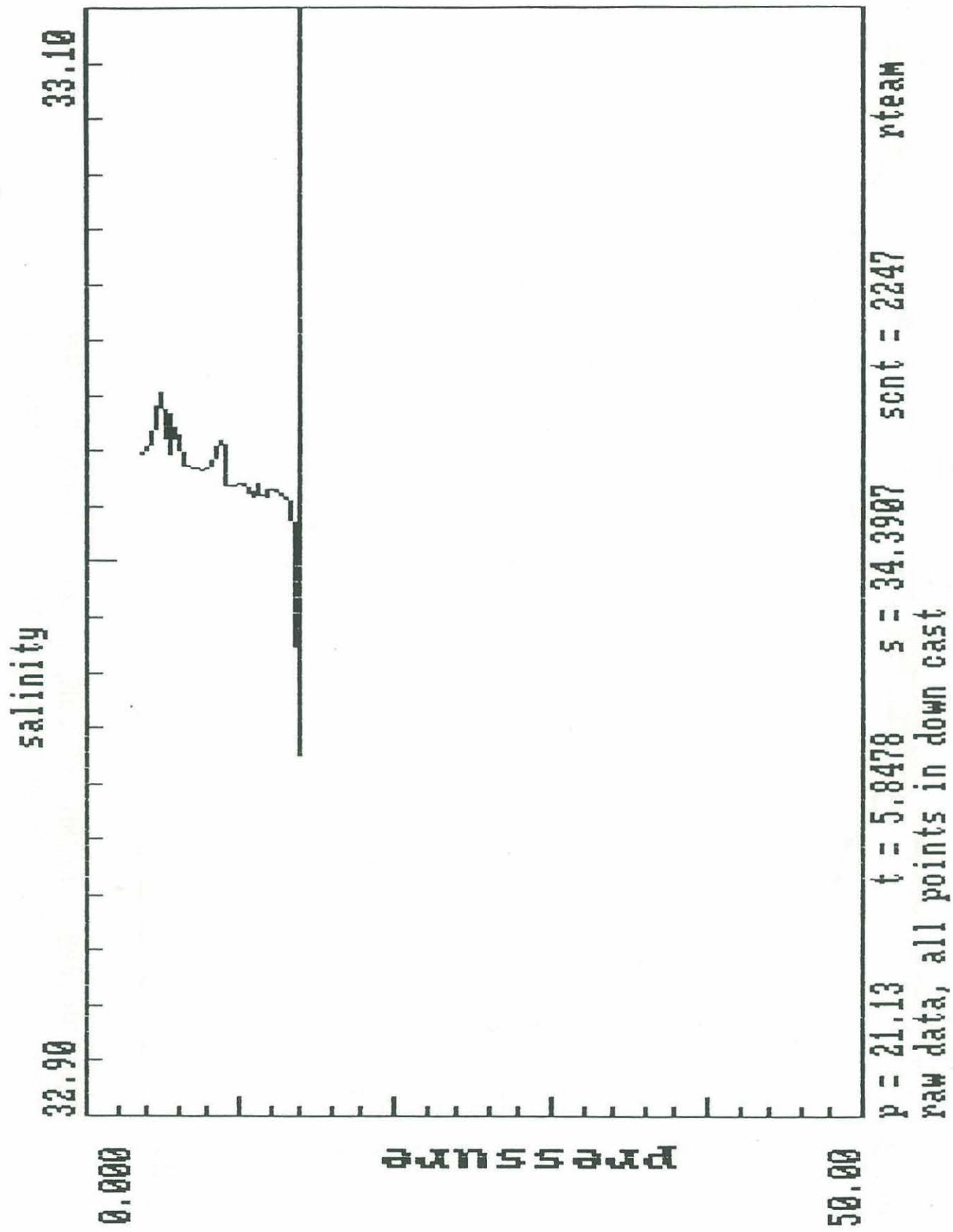
FIGURE 1 Salinity Versus Pressure For Just The Top 50m, No Averaging
