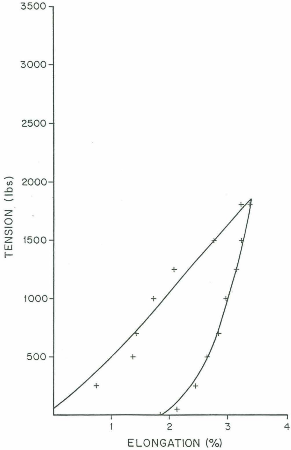
Figure 2.3 Spectra Stress/Strain Curve - Rope #2
