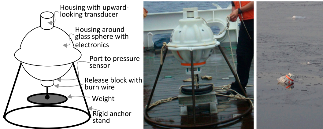
FIG. 2. (left) PIES schematic, (middle) PIES on deck, ready for deployment, and (right) awaiting retrieval from the sea surface after a mission. The rigid anchor stand and weight are not retrieved on recovery.
