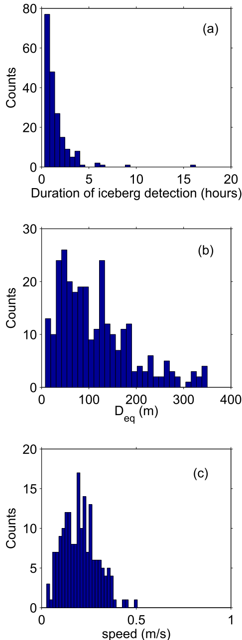
FIG. 12. Statistics of iceberg detections. (a) Duration of iceberg detections for the 195 cases when there was clearly only one iceberg keel within the IES's detection volume. During most of the remaining 90 detection events, it appears likely that one iceberg did not exit the detection volume before another one entered; however, a single iceberg with a complicated keel shape cannot be ruled out for these cases. (b) Calculation of d_{eq} from the minimum \tau occurring during each of the total (285) detection events. (c) Drift speed for the 178 cases where speed could be determined (not every detection included in the top panel has a clear \tau_{min} or a well-defined slope on a \tau^2 vs t^2 plot, so d_{eq} and drift speed could not be determined for each detection of a single iceberg).
