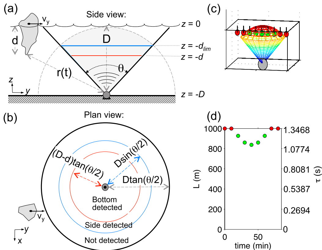
FIG. 3. (a) Schematic depicting a side view of the cone-shaped volume (inside the heavy black lines, indicating the approximate -3 -dB surface) ensonified by the four pings emitted during an IES burst. Also shown is a deep iceberg ( d > d_{lim} ) moving with drift speed v_y ( v_x = 0 ) that is about to enter the ensonified volume. (b) Plan view of the volume in (a) at the sea surface, where z = 0 (black circle), at z = -d_{lim} (blue), and at z = -d , the base of the iceberg keel (red). Labeled areas indicate regions where the iceberg can be detected as the iceberg moves through the ensonified cone. (c) Schematic of a shallow point iceberg (represented by the vertical black lines) progressively passing through the region ensonified by the IES. When the iceberg is within the detection volume, the deepest point on the keel bottom (indicated by the green dots) will be detected by the IES. (d) Corresponding reflection curve (for a case with D = 1000 m and \bar{c} = 1485 m s ^{-1} ): red dots denote reflections from the sea surface and green dots are successive reflections from the same (deepest) point on the bottom of the keel.
