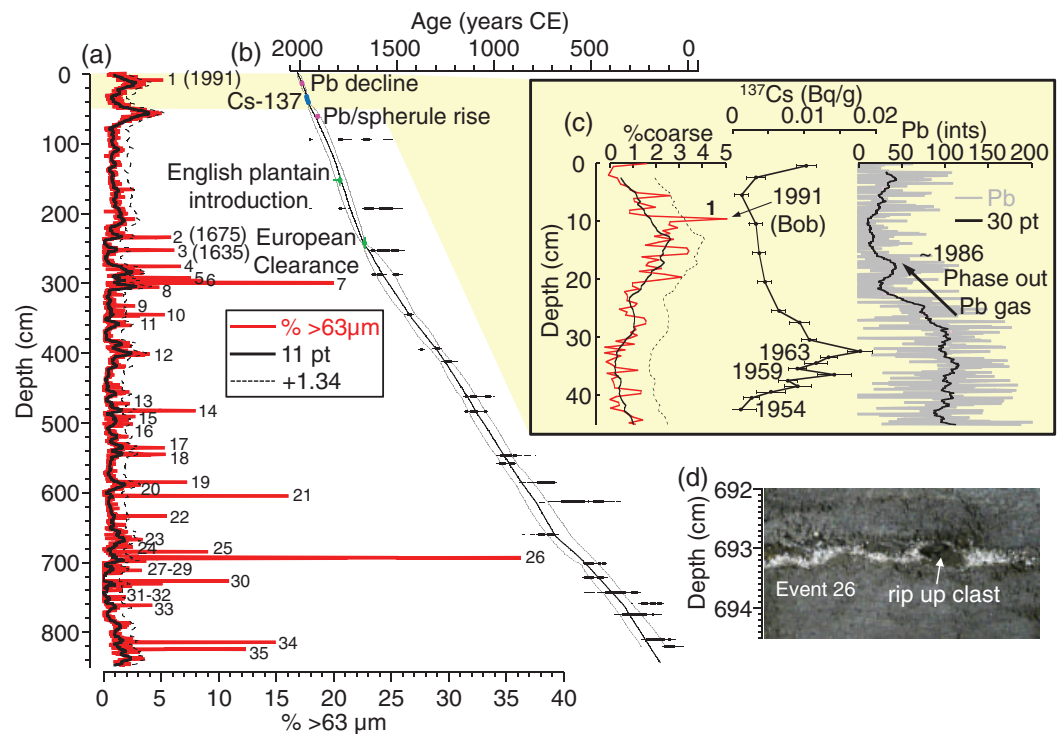
Figure 2. Overwash event record from Salt Pond, MA. (a) Percent sand fraction (>63 μm) results (red) from core collected from the deepest part of the basin (SP2) with 11-point running mean filter that excludes coarse fraction values exceeding 5% (black). Dashed line is event threshold of >1.34%. Events are numbered 1–35. (b) Age model derived from radiocarbon (2σ ranges thin bars and 1σ ranges thick bars; 95% confidence bounds shown around mean age; Supporting Information Table S1) and stratigraphic dates, including pollen evidence (green) of European land clearance and agriculture in the late seventeenth century and the introduction of English plantain in the early nineteenth century (Supporting Information Figure S5). 137 Cs activity provides ages related to nuclear weapons testing in the middle twentieth century (blue). Pb pollution and opaque spherules provide ages related to industrialization (purple). (c) Blow up of the upper 45 cm of percent sand fraction data with 137 Cs and bulk Pb pollution chrono-horizons. The event bed attributed to Hurricane Bob is noted. This portion of the record is replicated in core SP6 (Supporting Information Figure S6). (d) Photograph of event bed 26 at 693 cm.
