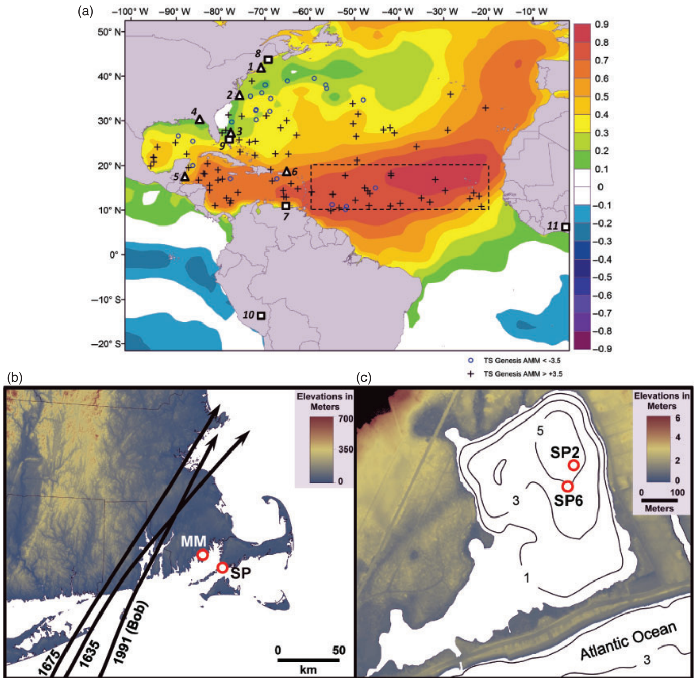
Figure 1. Location maps. (a) Correlation map of boreal summer SST and AMM. SSTs are warmer during positive AMM. Triangles show locations of paleo-hurricane reconstructions presented here (1—Salt Pond [this study] and Mattapoisett Marsh [Boldt et al., 2010]; 2—Outer Banks inlets [Mallinson et al., 2011]; 3—Thatchpoint Blue Hole [van Hengstum et al., 2013], 4—Mullet Pond [Lane et al., 2011] and Spring Creek Pond [Brandon et al., 2013]; 5—Lighthouse Blue Hole [Denomme et al., 2014]; 6—Laguna Playa Grande [Donnelly and Woodruff, 2007]). The MDR for North Atlantic tropical cyclones is noted in the dashed box. Locations of additional paleoclimate proxy records presented in Figures 4 and 5 are noted with squares (7—Cariaco Basin [Wurtzel et al., 2013; Haug et al., 2001]; 8—Gulf of Maine SST [Wanamaker et al., 2008]; 9—Bahamas SST [Saenger et al., 2009]; 10—Quelccaya Ice Cap [Thompson et al., 2013]; 11—Lake Bosumtwi [Shanahan et al., 2009]). Genesis locations for hurricanes forming in the most positive AMM (+) and most negative AMM (o) years are shown. Note the increase in genesis off the North American east coast in negative AMM. (b) Location of Salt Pond (SP) and Mattapoisett Marsh (MM) [Boldt et al., 2010] in southeastern New England and approximate tracks of historical hurricanes thought to have left a coarse event bed in Salt Pond sediments. (c) Map of Salt Pond showing core locations (SP2, SP6) and bathymetry and topography in meters.
