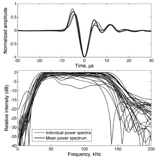
Fig. 3: Stenella frontalis echolocation clicks: A: Waveform of the 4 echolocation clicks of highest amplitude. Waveforms (sample rate 500 kHz) are upsampled (x10 low-pass interpolation), phase-aligned and normalised to the largest pressure excursion for easier comparison. B: Individual log-transformed power spectra (black lines) and mean Stenella frontalis energy distribution (grey dashed line) derived from all on-axis echolocation clicks. Power spectra are constructed using a 320-point fast Fourier transform based on a 32-point (64 \mu s) window (resulting in x10 sinc interpolation) centered on the peak envelope of each click. Note that the flatness of the mean energy distribution is partly a result of differences in peak frequency between clicks, whereas individual power spectra exhibit much more spectral variation.
