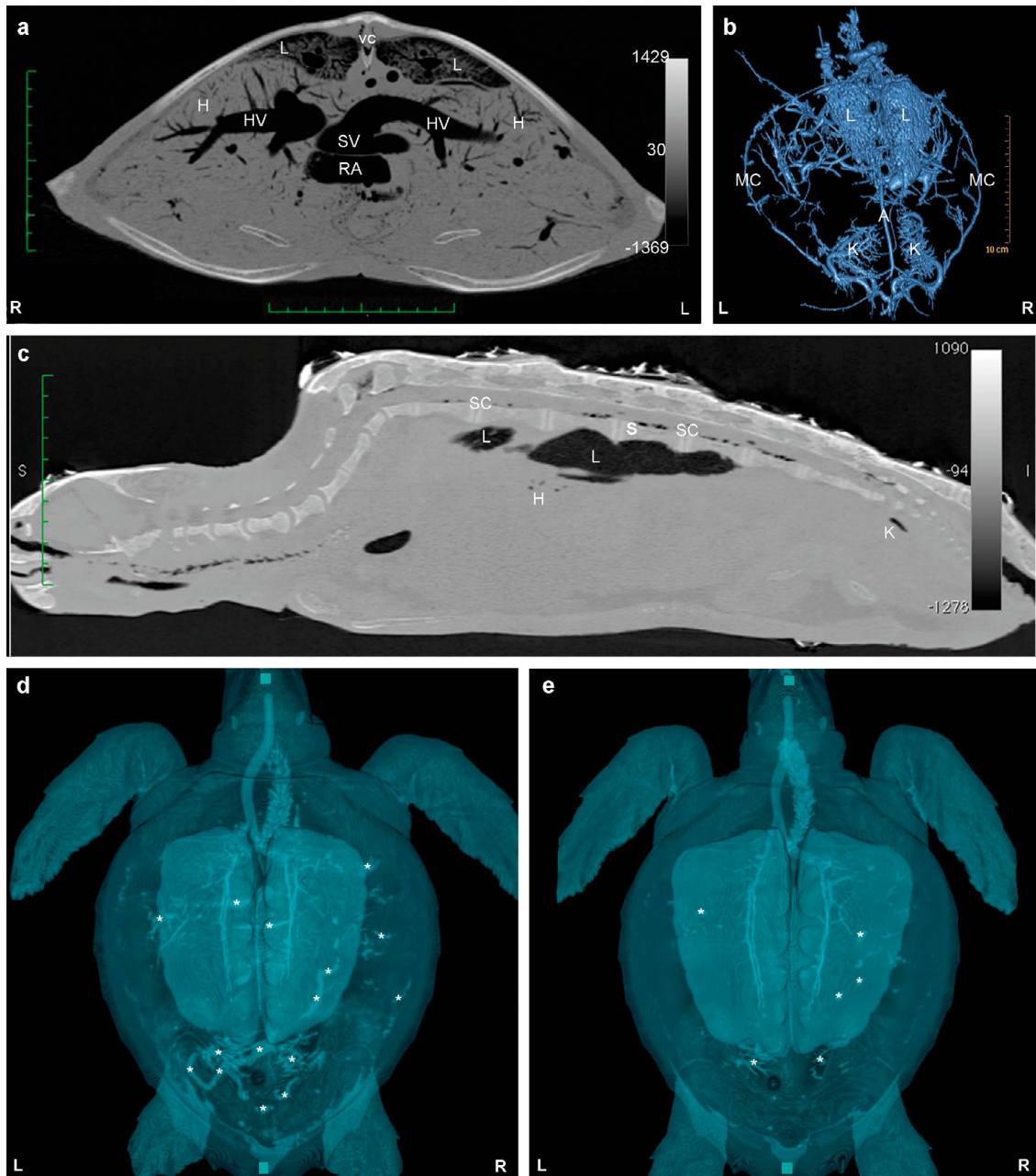
Fig. 2. Evidence of gas embolism (GE) in loggerhead sea turtles Caretta caretta on computed tomography. (a) Transverse image of mid-cranial coelomic region at the level of the heart in case CcGE15 (severe systemic GE), showing evidence of intraluminal gas (black) inside the heart and major vessels. Gas is also present within the venous hepatic system (H) and vertebral canal (VC). Lungs (L) are hyperattenuated (whiter) due to partial collapse. HV: hepatic veins; SV: sinus venosus; RA: right atrium. (b) Dorsal oblique view of 3D volume recreation through volumetric segmented reconstruction (volume rendering) in the same turtle. Note the presence of gas within the different peripheral and intracoelomic vessels. Lungs contain less gas than normal. The kidneys (K) are clearly visualized due to the massive presence of intravascular gas in this region. A: aorta; MC: marginocostal vein. (c) Mid-sagittal image of case CcGE20 (mild systemic GE). Note presence of abnormal gas in the central nervous system, spinal cord (SC), and renal and minor hepatic vessels. (d,e) Dorsal views of 3D air volume rendering view of total gas volume inside CcGE23 (moderate systemic GE) before (d) and after (e) oxygen hyperbaric treatment for recompression. Images were obtained 6 h apart. All gas is shown in brighter color, and intravascular gas is marked with asterisks. In (d), note the delineation of hepatic veins and renal vessels by the presence of intraluminal gas before treatment. Lung expansion is also reduced. In (e), most gas contained in the large vessels has almost disappeared after hyperbaric treatment, indicating gas reabsorption/elimination, while pulmonary expansion is back to normal. Few minor vessels still contain gas in the periphery of the hepatic and renal projection areas
