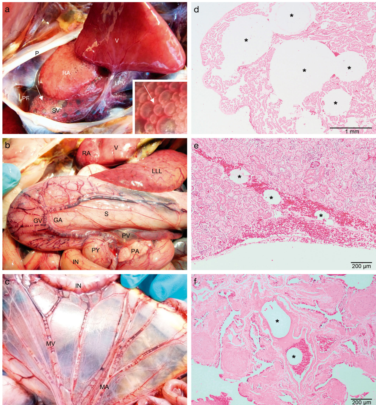
Fig. 3. (a–c) Gross and (d–f) histopathological findings in loggerhead sea turtles Caretta caretta . (a) Caudo-ventral view of the heart, dorsal surface, of case CcGE18 (mild/moderate systemic gas embolism, GE). The right atrium (RA) and sinus venosus (SV, amplified in inset) are diffusely distended with a moderate amount of intracameral gas bubbles. V: ventricle; LA: left atrium; LPV: left precaval vein; P: pericardium; PF: pericardial fluid. (b) Left dorso-lateral view of the stomach (S) greater curvature (after being reflected cranially) and liver left lobe (LLL) of case CcGE14 (moderate systemic GE). Note that gastric veins (GV) from greater curvature and the pyloric vein (PV) are diffusely expanded with variably sized gas bubbles. GA: gastric artery; PY: pylorus; PA: pancreas. (c) Small intestine (IN) and mesentery (MA/MV: mesenteric artery/vein) of case CcGE14. Note that mesenteric veins are diffusely expanded with a large amount of variably sized gas bubbles, coalescing at the mesenteric venous root. (d) Right atrium of case CcGE15 (severe systemic GE). Atrial lumen shows multifocal to coalescing, variably sized, round to oval, fat-negative gas emboli (asterisks), compressing the adjacent myocardium. H&E stain. (e) Kidney of case CcGE18 (mild/moderate GE). Interrenicular veins are multifocally occupied by round to oval, variably sized, fat-negative gas emboli. H&E. (f) Lung of case CcGE7 (severe systemic GE). Pulmonary veins show intravascular, variably sized, round to oval, fat-negative gas emboli. H&E
