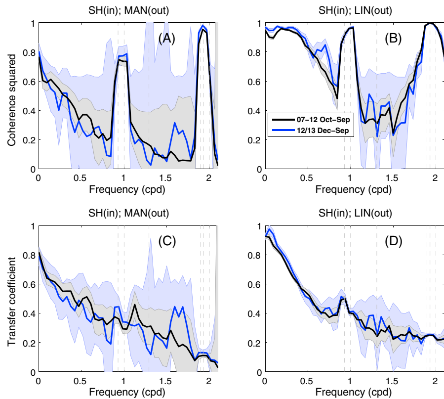
Figure 4. (a and b) Water level coherence and (c and d) transfer function between SH and MAN and between SH and LIN for the October to September period for 2007–2012 (pre-Hurricane Sandy) and December to September 2012–2013 (post-Sandy). The shaded areas denote uncertainty envelopes for coherence and transfer function [Bendat and Piersol, 1986]. SH data are the input spectrum, and MAN and LIN are output spectra.
