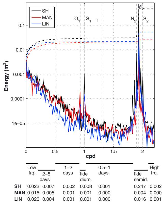
Figure 3. Energy spectra at SH, MAN, and LIN (solid lines) and cumulative energy (dashed lines). O_1 , S_1 , N_2 , M_2 , and S_2 label the principal tidal frequencies and “f” the inertial frequency. Values at the bottom is the sum of energy ( m^2 ) at SH, MAN, and LIN in low frequency, 2–5 days, 1–2 days, diurnal tide, 0.5–1 day, semidiurnal tide, and high-frequency bands. (cpd: cycles per day).
