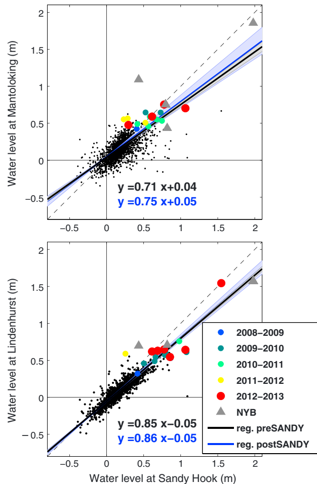
Figure 5. Scatterplot of daily maximum subtidal (DMS) water level in back-barrier bays at MAN and LIN versus coastal sea level at SH (NYB data (triangle markers) was used when SH was down). The DMS water levels associated with the 20 highest daily high-water events at LIN and MAN (Table 1) are shown as larger dots and colored by year with the post-Hurricane Sandy events marked with larger red dots. Dashed line is 1:1, and the pre-Sandy (black) and post-Sandy (blue) robust regressions are indicated with solid lines (formula shown), and shading is the 95% confidence bounds.
