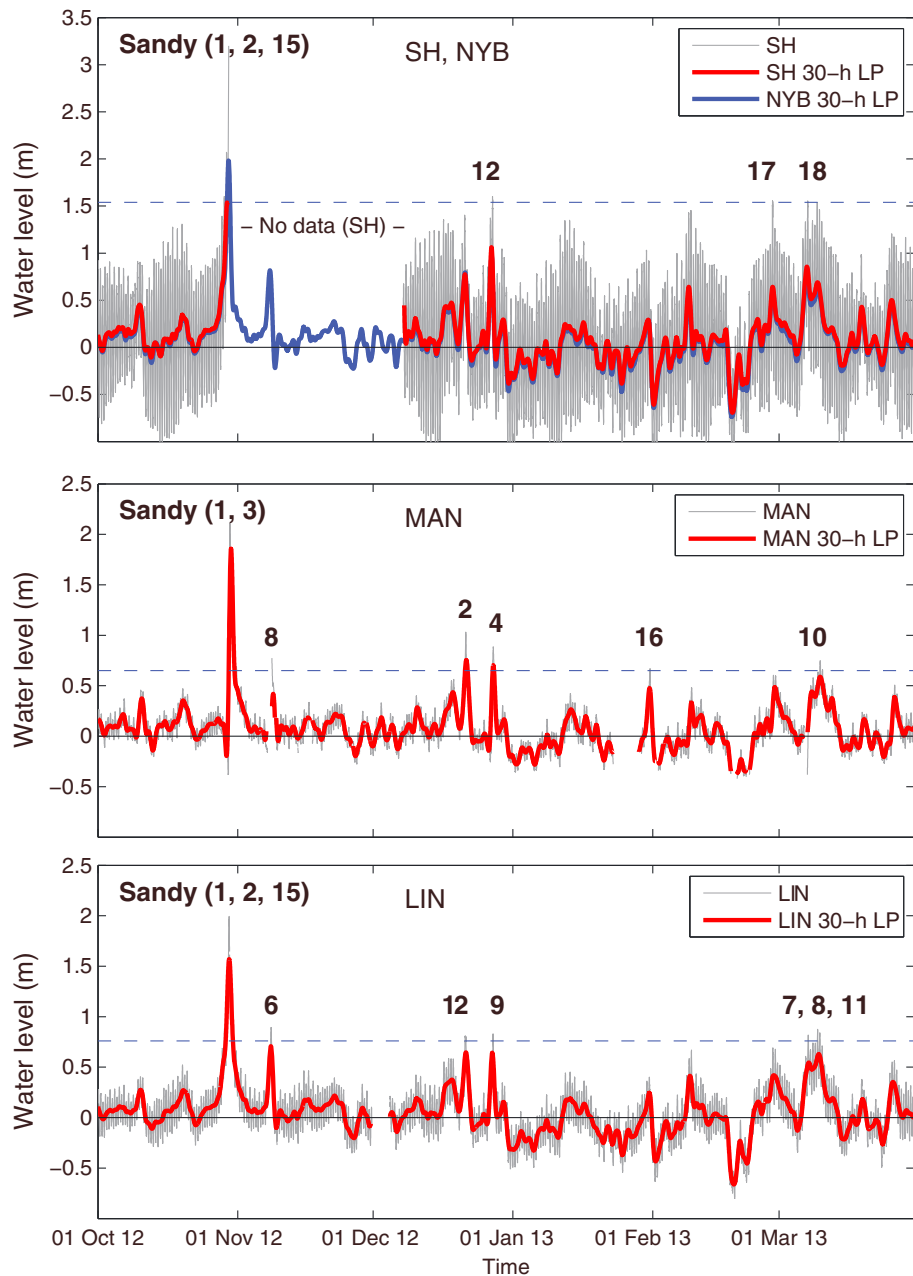
Figure 2. Time series of 6 min (gray) and 30 h low-pass filtered (red) sea level at SH, MAN, and LIN for October 2012 to April 2013. Low-pass filtered sea level at NYB (blue) included on SH plot. Numbers are the event rank for the top 20 daily high-water events since 2007 (Table 1), and the blue dashed lines are the event thresholds at each station. High-water events following Hurricane Sandy occurred on 8 November, 21 December, and 27 December 2012 and 31 January and 7 March 2013 (weather maps for these events are in Figure S2 in the supporting information). Events labeled with multiple numbers indicate a record water level occurring on successive days.
