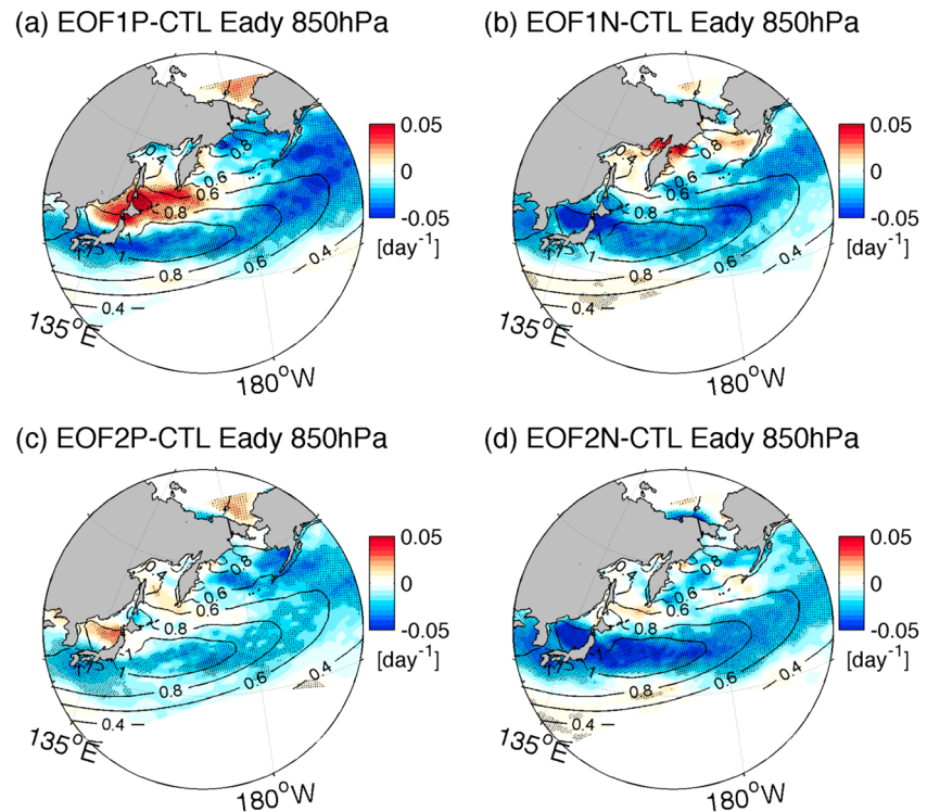
Figure 16. (a–d) Equilibrium NDJFMA response in the Eady growth rate ( \sigma , [ \text{day}^{-1} ], shading) at 850 hPa overlaid with the climatological mean 850 hPa \sigma (black contours, Cl = 0.2 \text{ day}^{-1} ). Dots denote the areas of significant ( p = 0.05 ) change.
