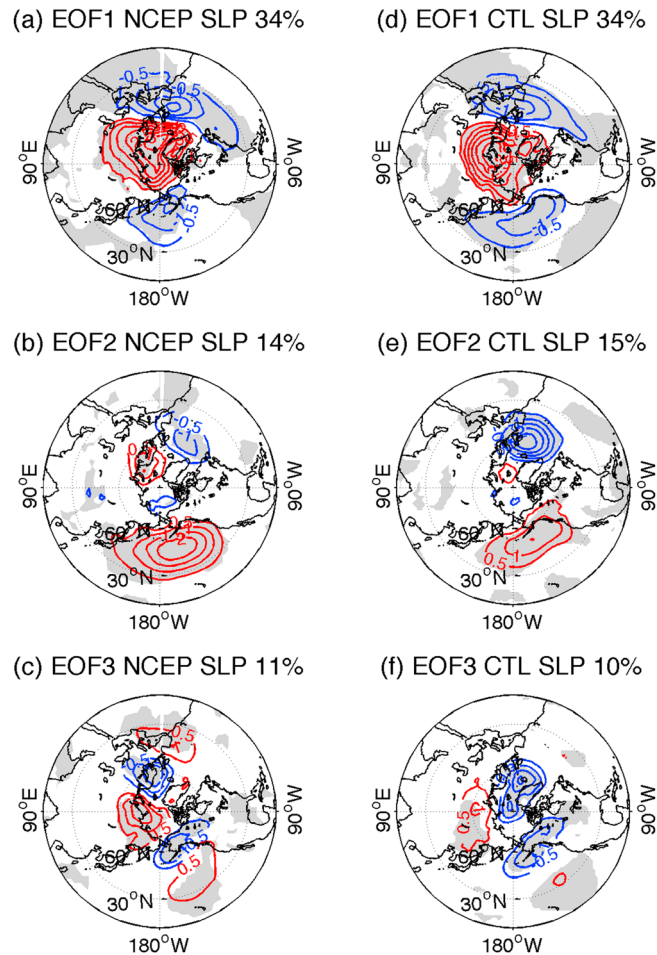
Figure 3. Leading EOF patterns of the NDJFMA-averaged SLP (hPa), contours, positive red, negative blue for (left) the 40 year NCEP-NCAR Reanalysis (NCEP hereafter) from 1970 through 2009 and (right) the 40-member ensemble CTL simulation. The influence of the tropical SST variability is removed in the NCEP SLP fields via regression prior to EOF analysis as explained in the text.
