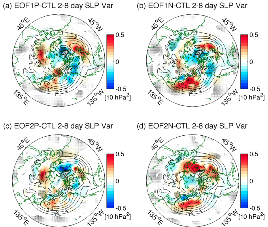
Figure 14. (a–d) Equilibrium NDJFMA response in the variance of 2–8 day filtered SLP ( [hPa^2] , shading) overlaid with the variance of 2–8 day filtered SLP in CTL (black contours, CI = 10 hPa^2 ). Dots denote the areas of significant ( p = 0.05 ) response in the 2–8 day SLP variance.
