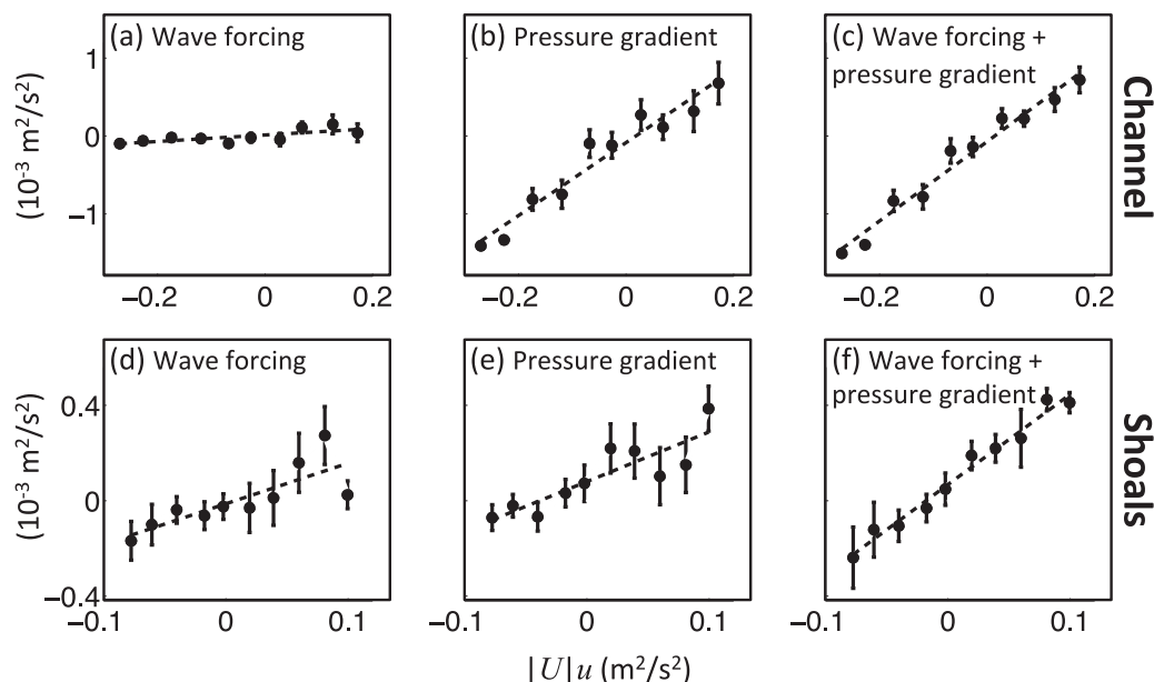
Figure 7. Binned means (circles) and standard deviations (vertical bars) of along-inlet (a and d) wave radiation-stress gradients, (b and e) pressure gradients, and (c and f) sum of along-inlet wave radiation-stress and pressure gradients versus inlet flow ( |U|u ) in the (a–c) channel and on the (d–f) shoals. The dashed lines are least squares linear fits to the binned values. Drag coefficients C_D calculated from the linear fits are 0.005 in the channel (Figure 7c) and 0.004 on the shoals (Figure 7f). Note the vertical ranges are larger for the channel (Figures 7a–7c) than for the shoals (Figures 7d–7f).
