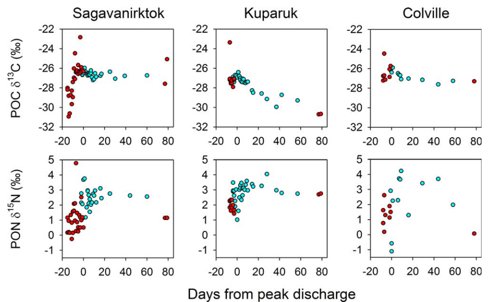
Figure 7. Temporal variations in \delta^{13}C and \delta^{15}N values particulate organic matter in the Sagavanirktok, Kugaruk, and Colville rivers. Data from 2006 (blue) and 2007 (red) are plotted relative to the timing of peak discharge (day 0) for each year.
