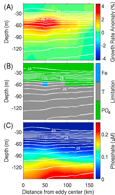
Figure 7. (a) Diazotrophic-specific growth rate anomaly, (b) limitation factors, and (c) phosphate concentrations in anticyclones with high diazotrophic biomass located within the white rectangle in Figure 6 (30–35° N, 30–48°W) during August–September. Two such features are identified by magenta dots in the snapshot shown in Figure 6. Radial averages were constructed from synoptic snapshots of model output using local maxima in sea level anomaly to define the positions of eddy centers. In each panel, density ( \sigma_\theta ) contours are overlaid in white.
