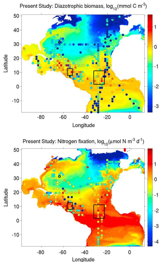
Figure 2. Simulated near-surface (0–10 m) (top) diazotrophic biomass and (bottom) nitrogen fixation. Data from Luo et al. [2012], binned onto the 1.6^\circ model grid, are shown as colored circles. Outlined in black are the locations of BATS (circle near 32^\circ\text{N} , 64^\circ\text{W} ), as well as tropical west (rectangle centered at 10^\circ\text{N} , 54^\circ\text{W} ) and tropical east (rectangle centered at 6^\circ\text{N} , 28^\circ\text{W} ) domains, for which detailed flux diagnosis is presented in Figure 4.
