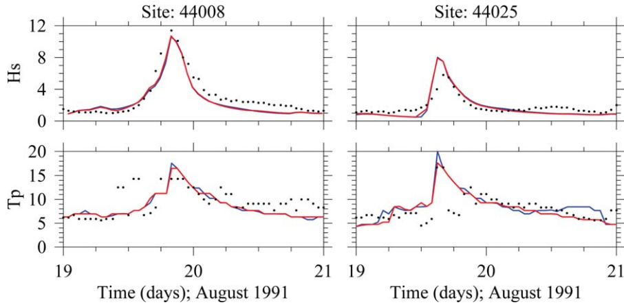
Figure 5. Comparisons between model-computed and observed significant wave heights and peak periods during 19–21 August 1991 at Buoy 44008 and 44025: observed (black dots); calculated without inclusion of wave-current interaction (red line); and calculated with inclusion of wave-current interaction (blue line).
