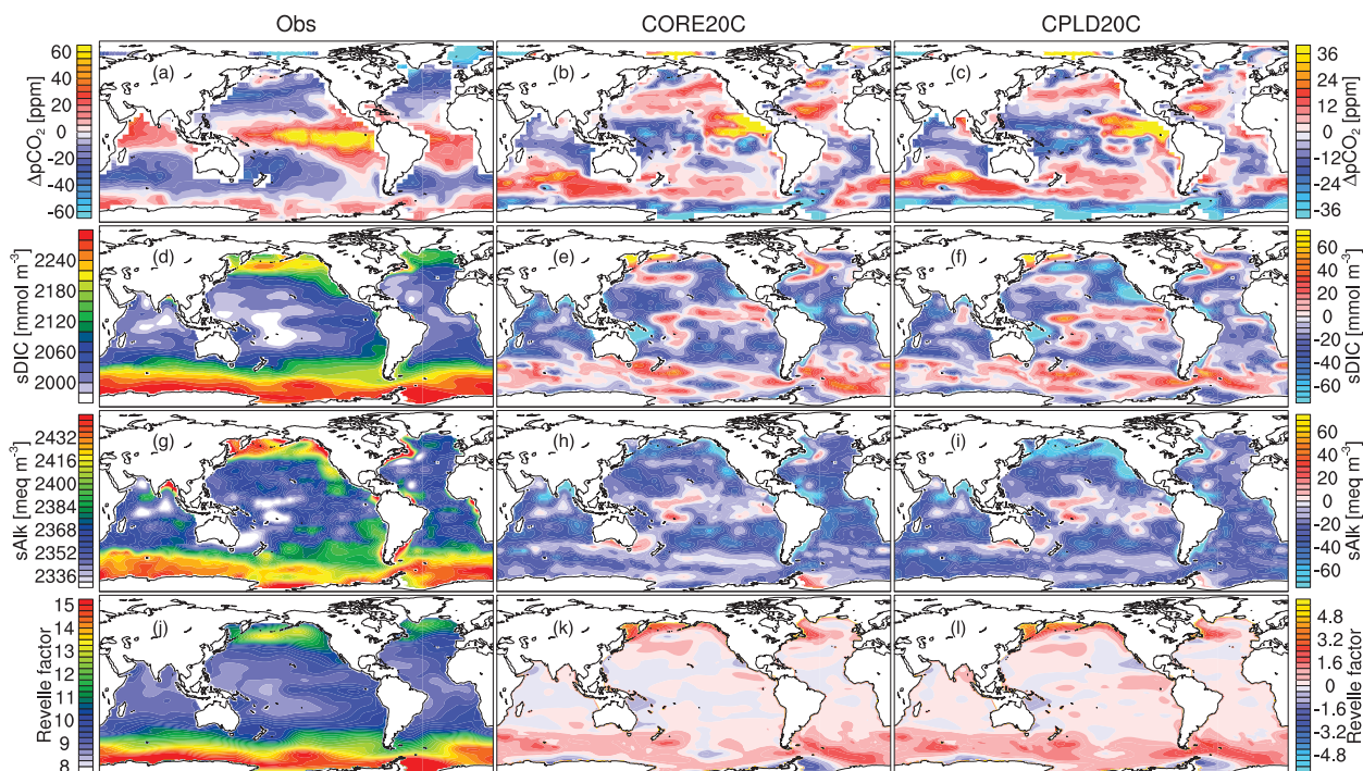
FIG. 1. (left) Observationally based climatologies of surface fields. Biases relative to observations in (center) CORE20C, and (right) CPLD20C. (a)–(c) Annual-mean sea–air p\text{CO}_2 difference ( \Delta p\text{CO}_2 ; Takahashi et al. 2009). (d)–(f) Salinity-normalized dissolved inorganic carbon, (g)–(i) salinity-normalized alkalinity, and (j)–(l) Revelle factor (Key et al. 2004). The Revelle factor was computed analytically from the thermodynamic equations.
