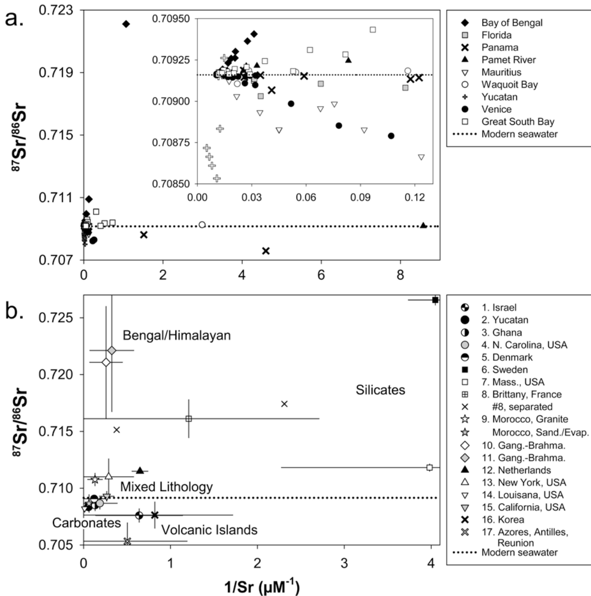
Figure 4. (a) Compiled ^{87}\text{Sr}/^{86}\text{Sr} data from the present study. The dashed line indicates the ^{87}\text{Sr}/^{86}\text{Sr} ratio of global average seawater. (b) Sr isotope ratios in diverse, near-coastal meteoric groundwaters. Common aquifer lithologies are indicated.
