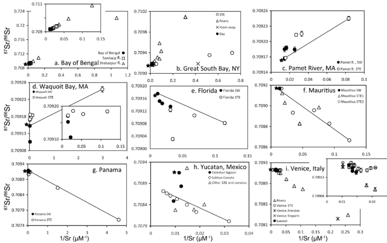
Figure 3. ^{87}\text{Sr}/^{86}\text{Sr} systematics. Symbols as in Fig. 2; star-shaped symbols indicate the approximate composition of global average seawater ( ^{87}\text{Sr}/^{86}\text{Sr} = 0.70916 , 1/\text{Sr} = 0.01 \mu\text{M}^{-1} ). Insets show expanded views near the origin. Diagonal lines indicate conservative mixing between meteoric groundwater and seawater end-members at the six STE sites where 3-endmember mixing was not indicated (i.e., excluding GSB and Venice). Isotope ratio uncertainties are drawn on these plots, but where error bars are not visible, they are smaller than the symbol size.
