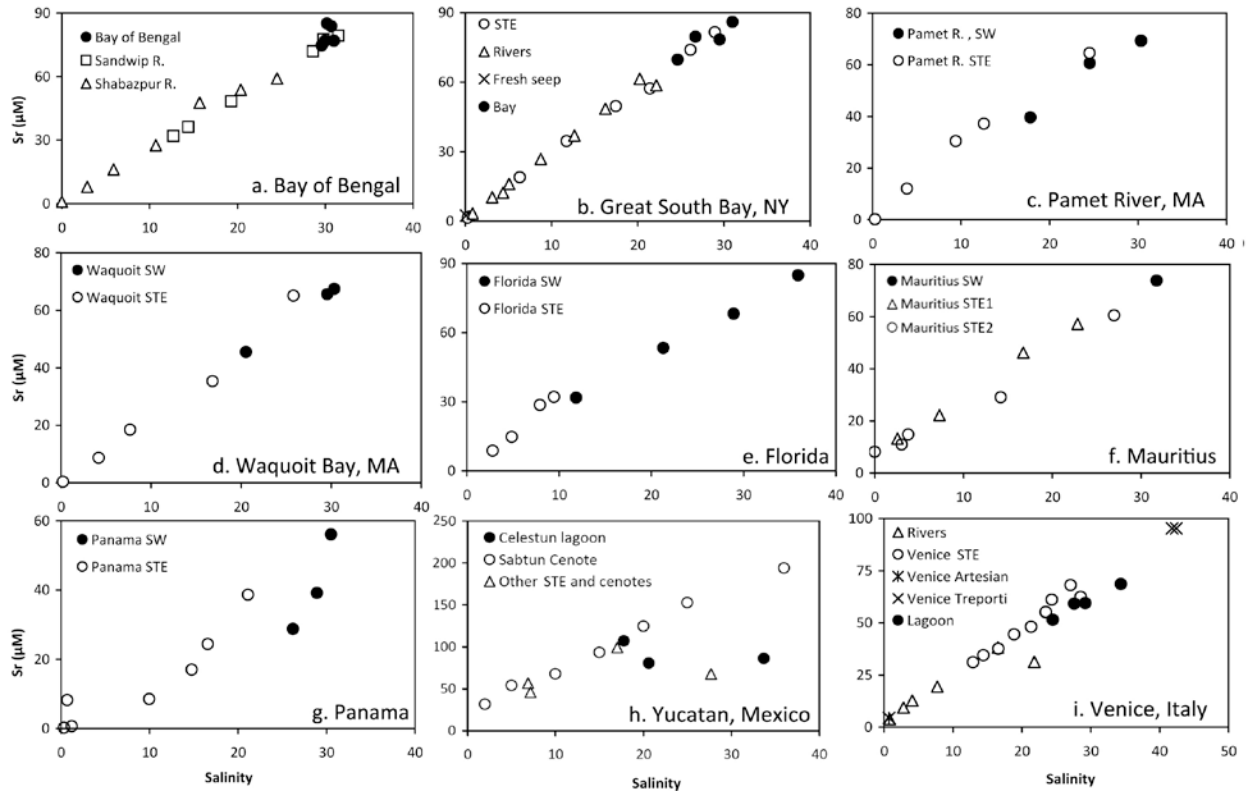
Figure 2. Co-variation of total dissolved Sr with salinity. Individual figure legends explain the symbols, and site locations are labeled on the graphs. Note that y-axis scales vary among the graphs.
