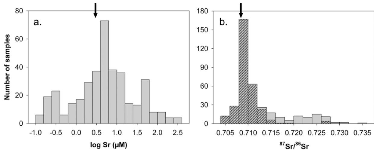
Figure 5. Frequency distribution of (a) log-transformed Sr concentrations and (b) ^{87}\text{Sr}/^{86}\text{Sr} ratios in global meteoric groundwaters (n = 381). Light-colored bars in (b) highlight samples from the unusually radiogenic Ganges-Brahmaputra region. Arrows indicate the flow-weighted global average groundwater composition based on the lithological model (2.9 \mu\text{M} Sr and ^{87}\text{Sr}/^{86}\text{Sr} of 0.7089). Data compiled from the current work and literature references cited in Fig. 4.
