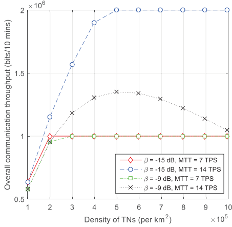
Fig. 4. Comparisons of overall throughput vs. TN density (FN density is 5000 km 2 ).
