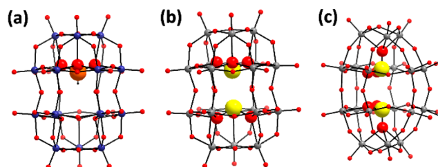
Figure 1. Structural representations of (a) [W^{VI}_{16}Mo^V_2O_{57}(XO_3)]^{10-} (X = HP for 1 , X = Se for 2 , X = Te for 3 ). (b) Peanut-shaped cluster [X_2W_{18}O_{60}]^{4-} (X = S, Se). (c) “Trojan-horse” type clusters [W_{18}O_{56}(XO_3)_2(H_2O)_2]^{8-} (X = S, Se, HP). Color scheme: P or Se or Te, orange; S, yellow; W/Mo V , indigo; W, gray; O, red.
