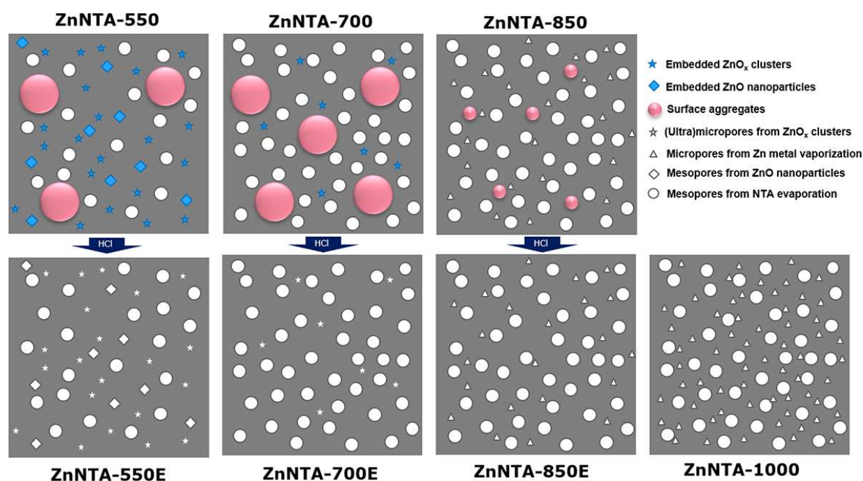
Scheme 2. Illustration of the effect of pyrolysis temperature and removal of in-situ generated Zn species on textural properties of carbons derived from ZnNTA mesocrystals.
