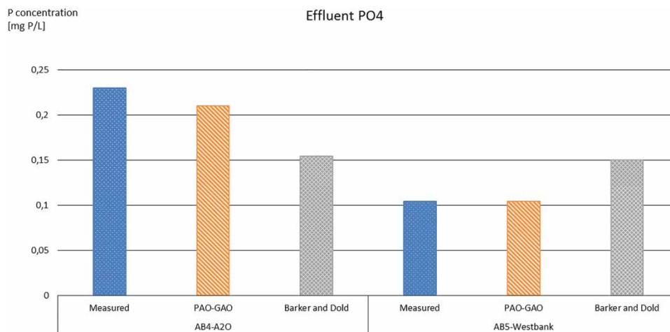
Figure 5 | Secondary effluent P concentrations.
