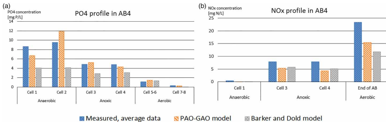
Figure 3 | Nutrient profiles in AB4 (a) PO4 profile; (b) NOx profile.
