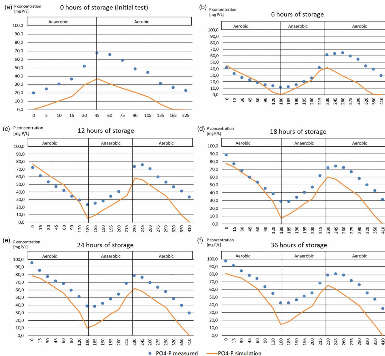
Figure 6 | (a–f) Phosphorus uptake and release tests with alternating aerobic/anaerobic periods after the indicated anaerobic storage period (X axis represents the time of the experiment in minutes).
