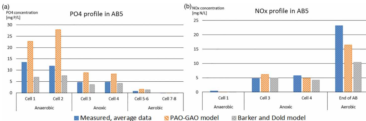
Figure 4 | Nutrient profiles in (a) PO4 profile; (b) NOx profile.
