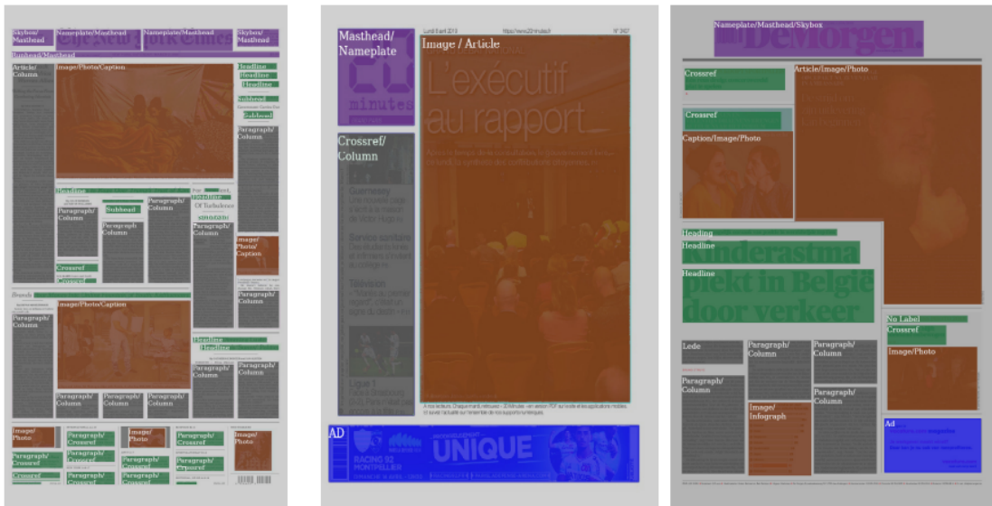
Figure 5: Visualization of the classification results on three different newspapers in our test set. Colors indicate primary categories as masthead elements (purple), text column (gray), ads (blue), images (brown) and minor text elements (green). Original images copyright of (from left to right) New York Times, 20 Minutes, and DeMorgan, courtesy of Newseum.
