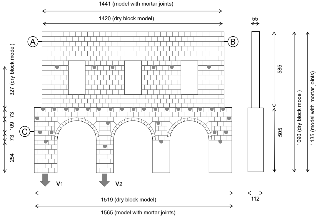
FIG. 3: Model dimensions (in mm), brick bond, location of amplified loads, applied displacements v_1 and v_2 and mechanical dial gauges a, b and c.
