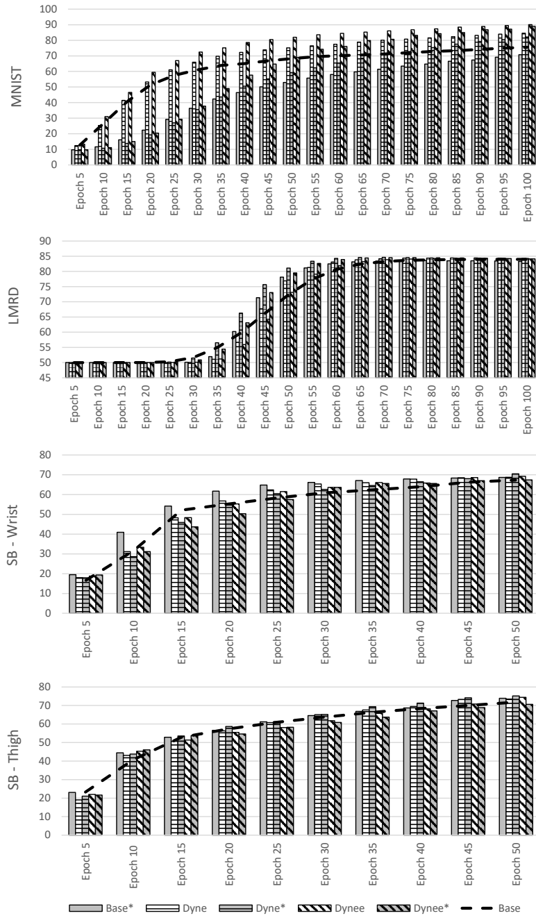
Fig. 2: Results on the MNIST, LMRD and SelfBACK datasets
