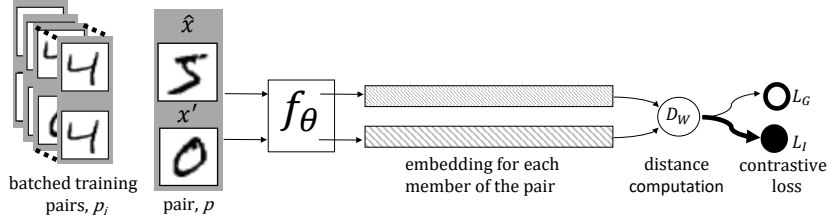
Fig. 1: The SNN learning process
