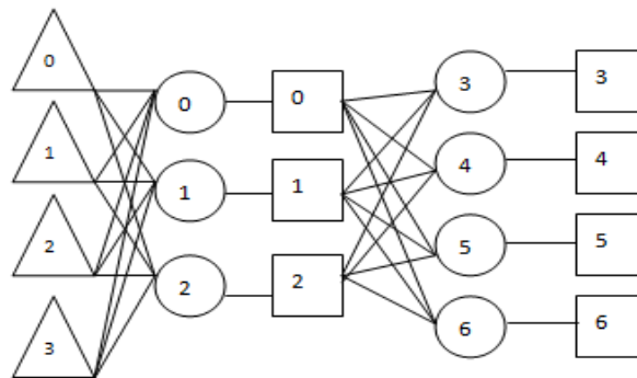
Fig. 3 The structure of the ARN used for pattern recognition experiments. The network consists of 4 inputs (triangles), 7 reaction units (circles) and 7 pools (squares). Each index of the input pattern array is fed into the corresponding input number. Output patterns are output at pools (squares) 3-6.
