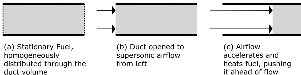
Fig. 9 A stationary gas impinged on by a supersonic flow.
