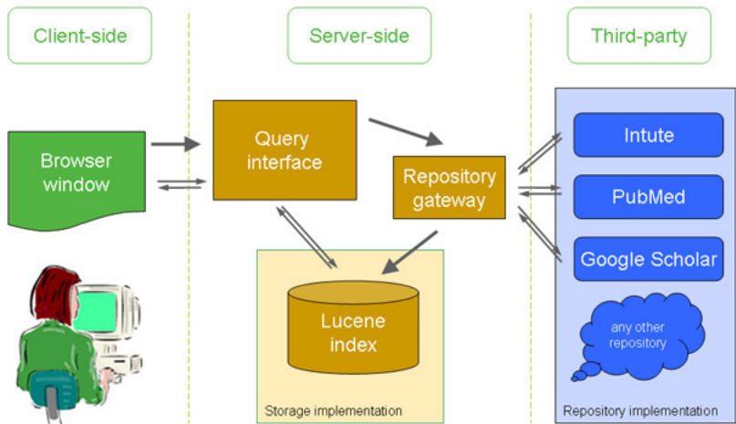
Figure 1: Architecture of DYNIXQ.
