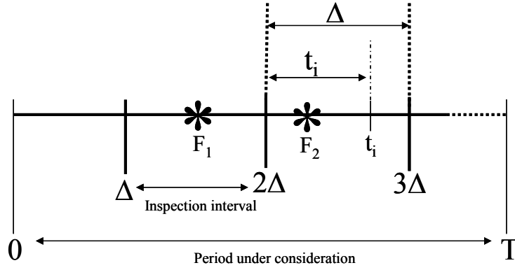
Figure 5 Delay-time concept
